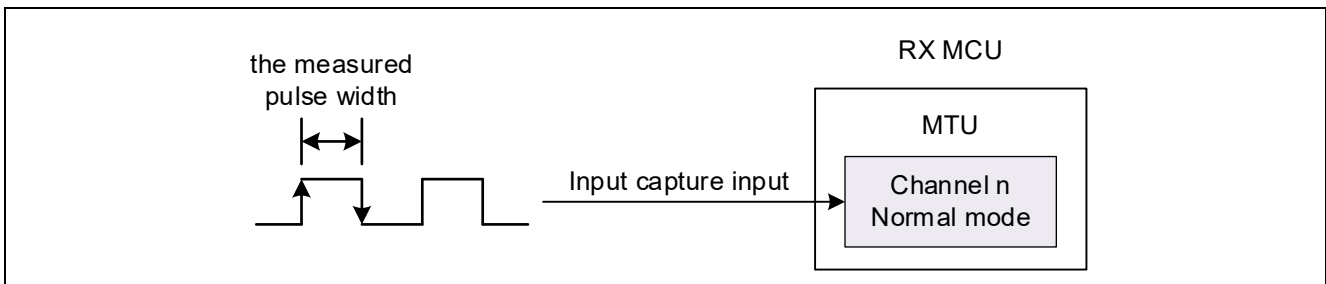
Figure 1.1 Pulse Width Measurement
