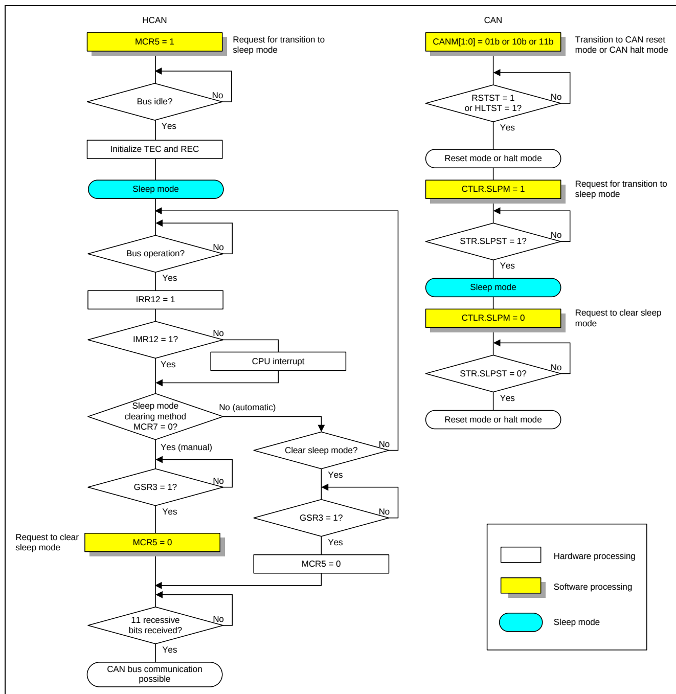
Figure 4.1 Sleep Mode Setting Procedure on H8S/2636 (HCAN) and RX65N (CAN)
