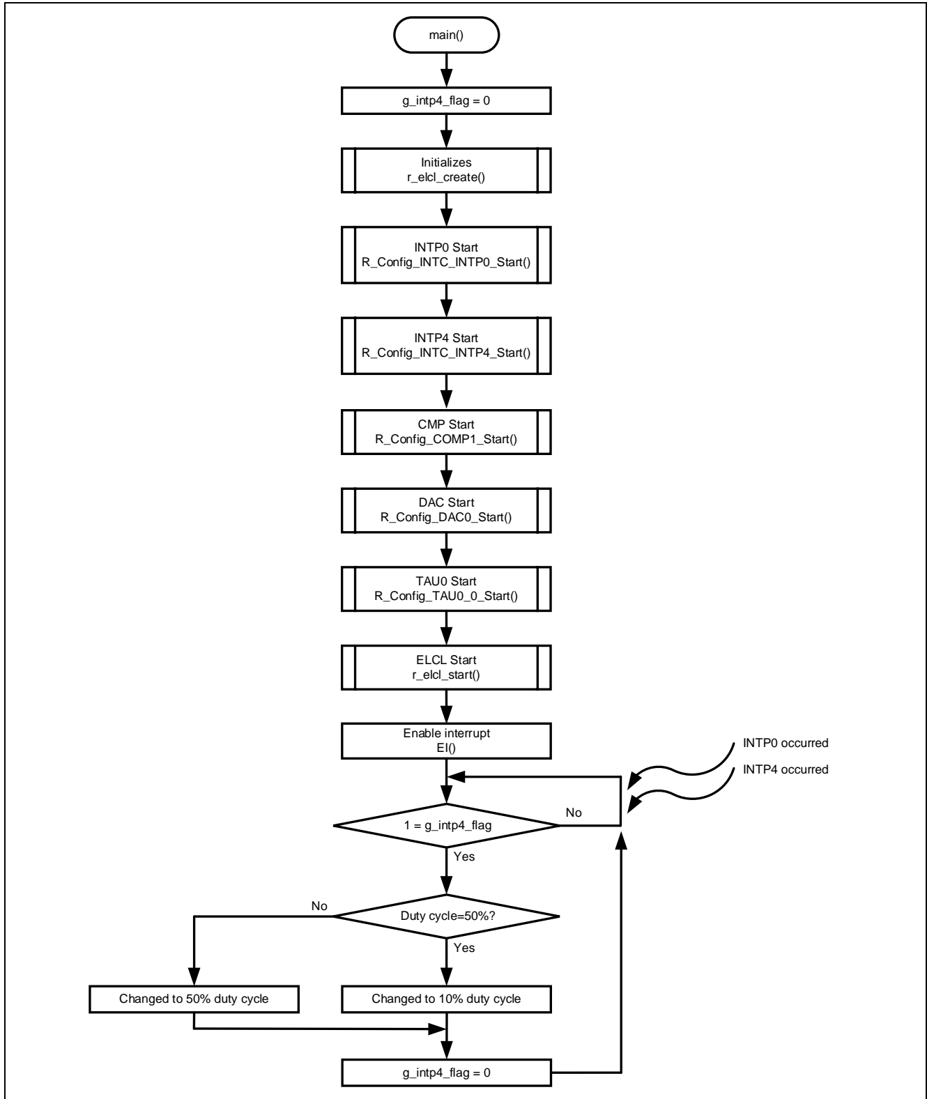
Figure 4-3 Main process
