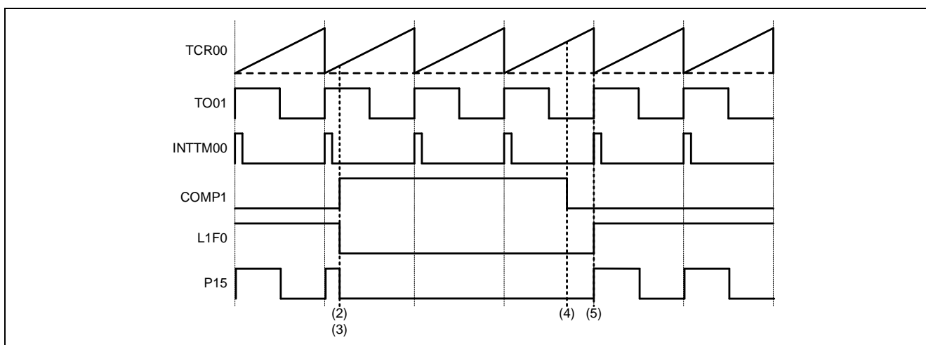
Figure 5-2 Timing chart
