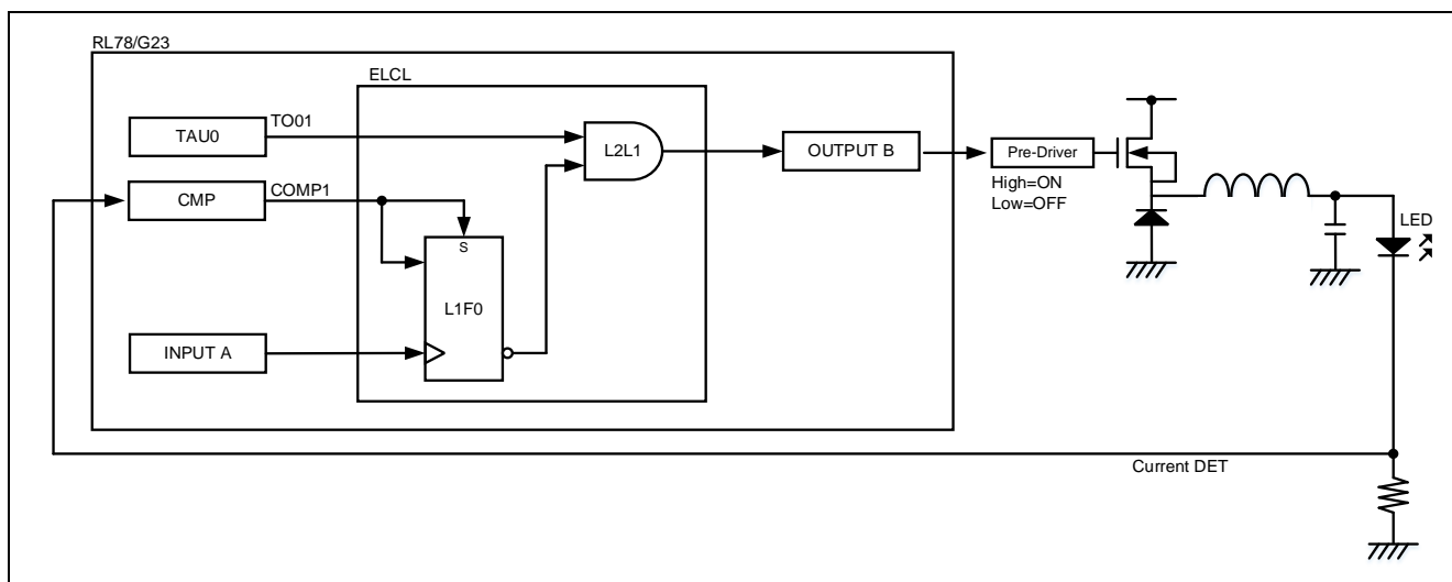
Figure 1-1 System Configuration
