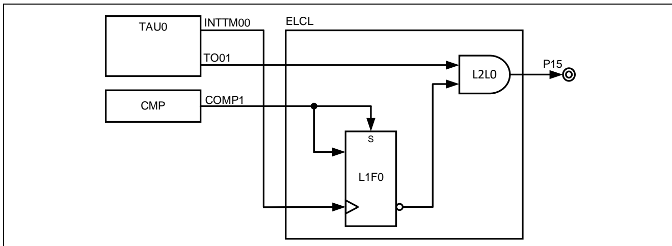
Figure 5-1 system configuration
