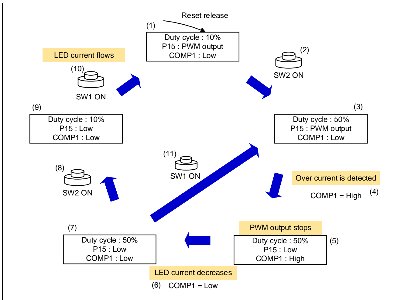
Figure 4-2 Operation overview
