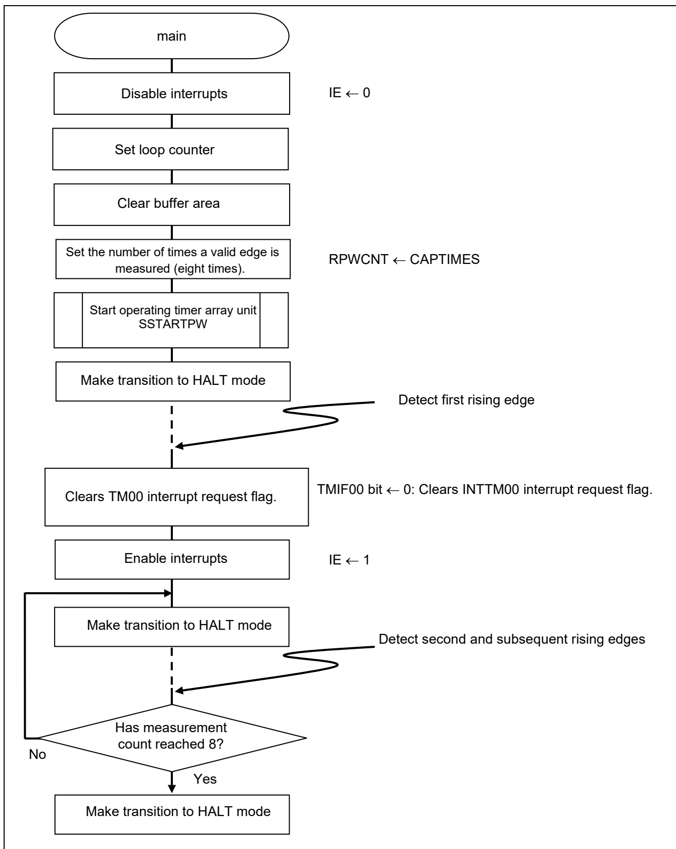
Figure 5.6 Main Processing
