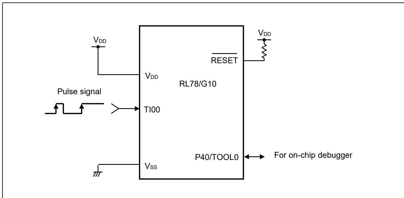
Figure 4.1 Hardware Configuration
