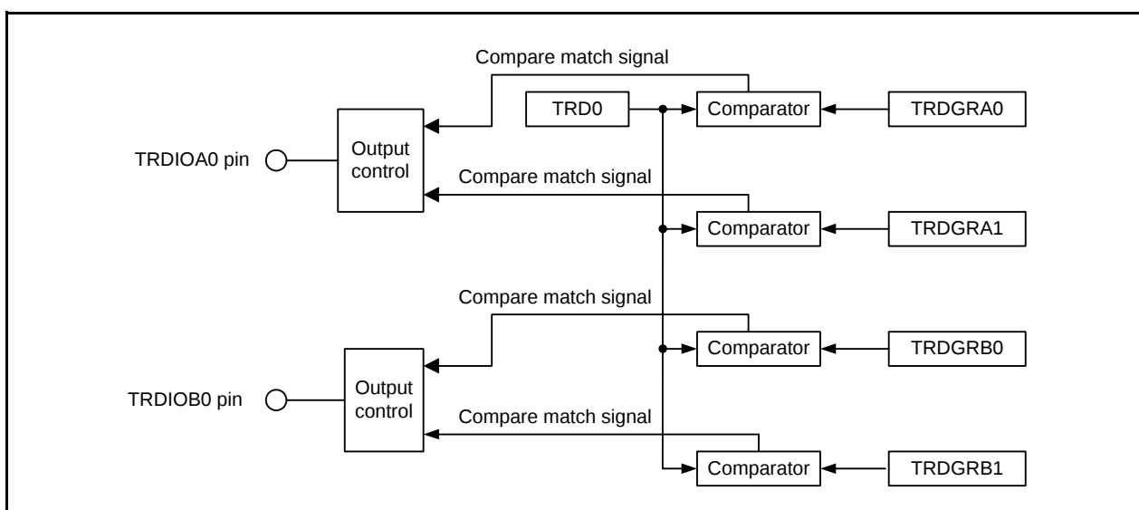
Figure 3.1 Block Diagram
