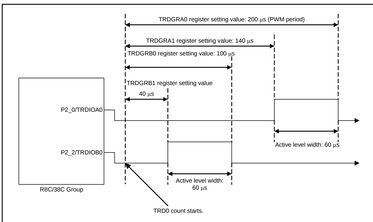
Figure 3.2 Timing Diagram
