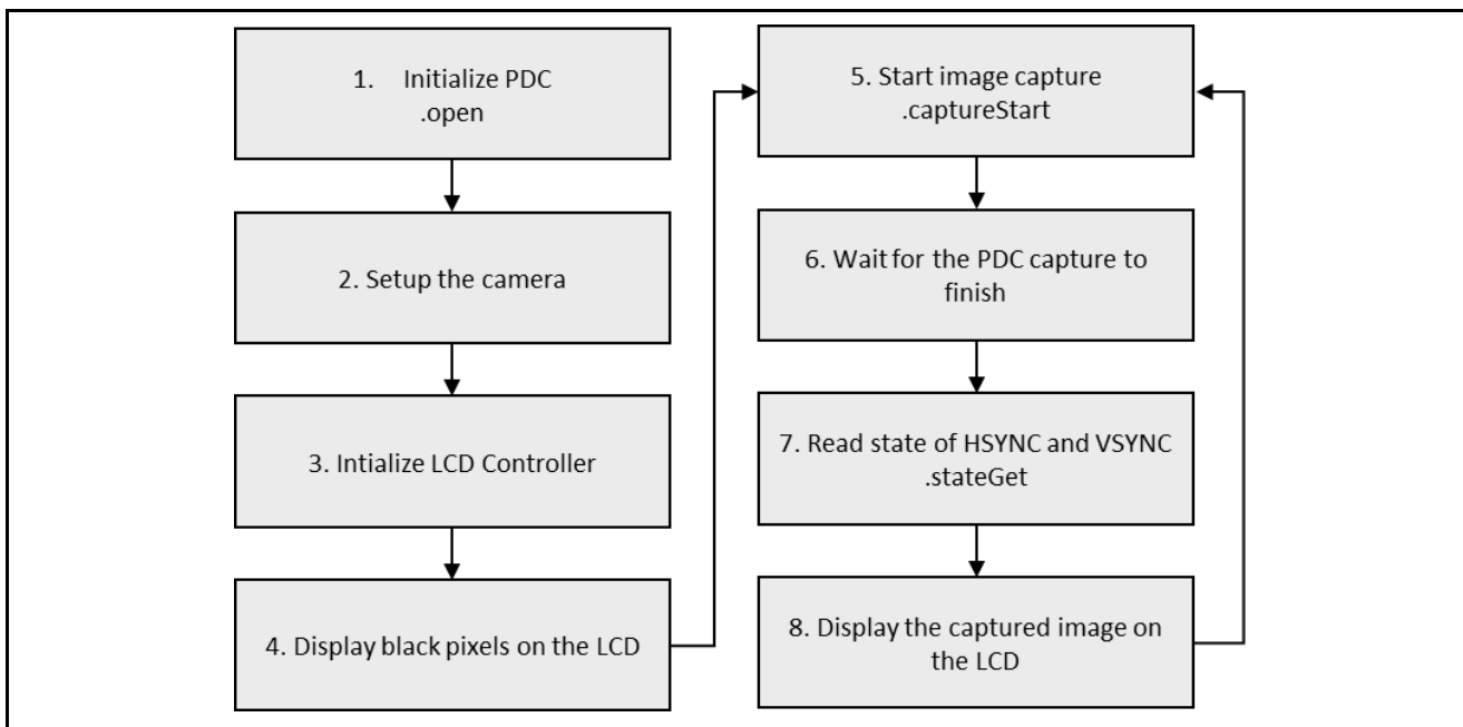
Figure 4. PDC HAL Module Application Project Flow Diagram
