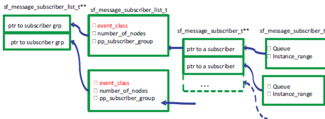
Figure 6. Message Framework — Subscriber List
