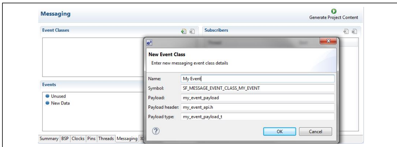
Figure 9. Messaging — e² studio New Event Class Configuration
