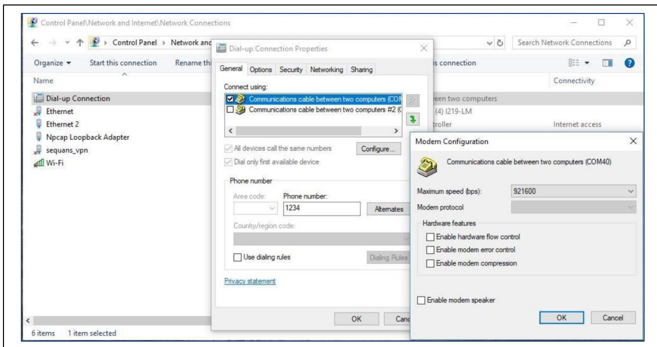
Figure 27. Configure Connection
