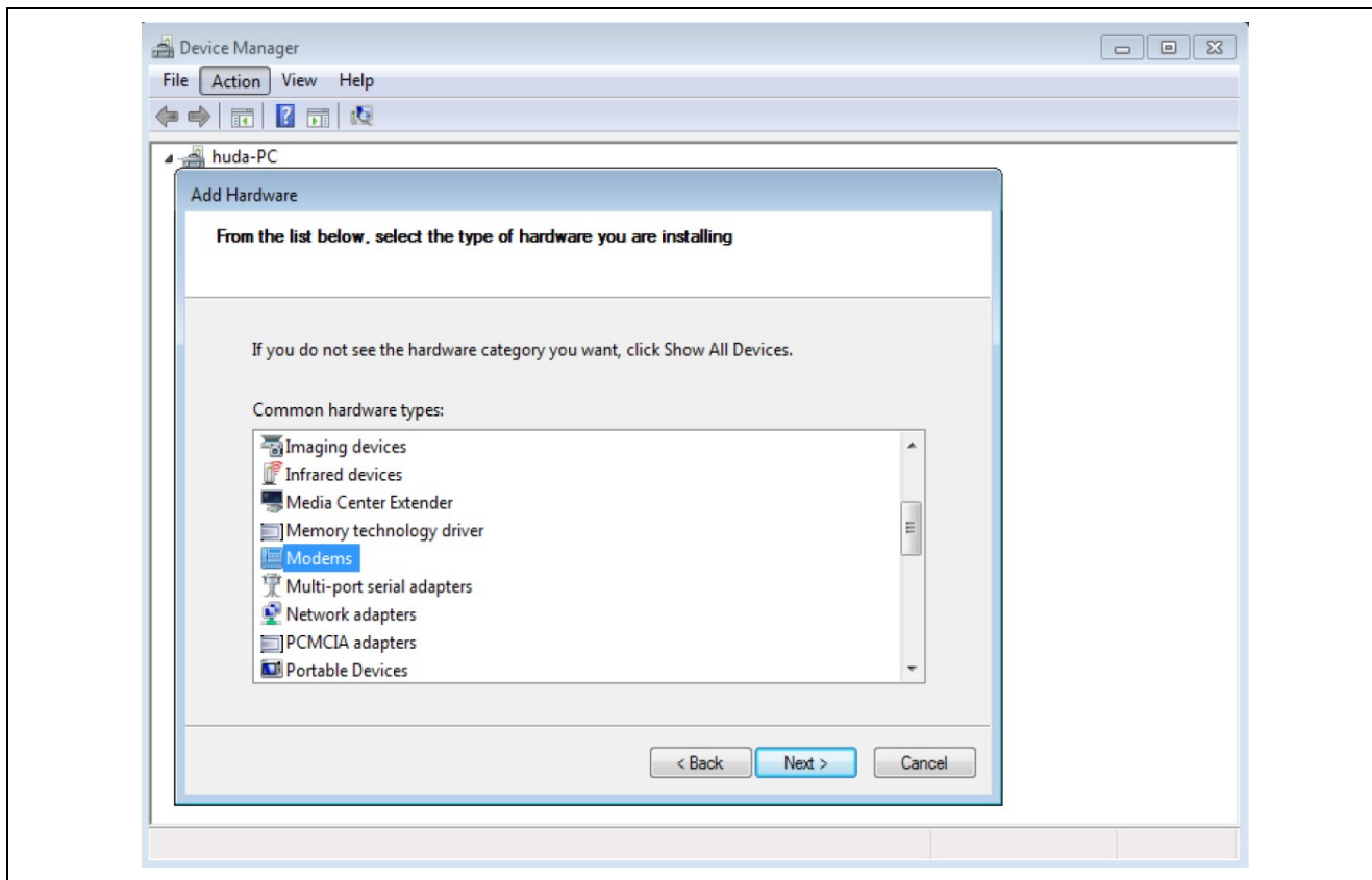
Figure 9. Select Modem
