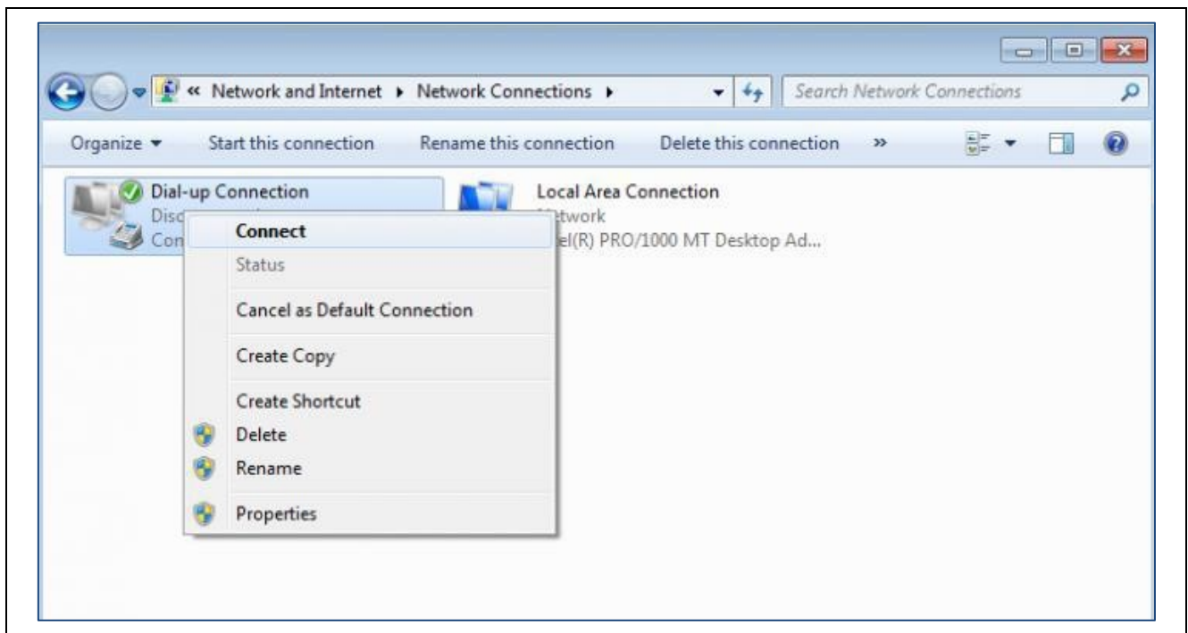
Figure 29. Connect
