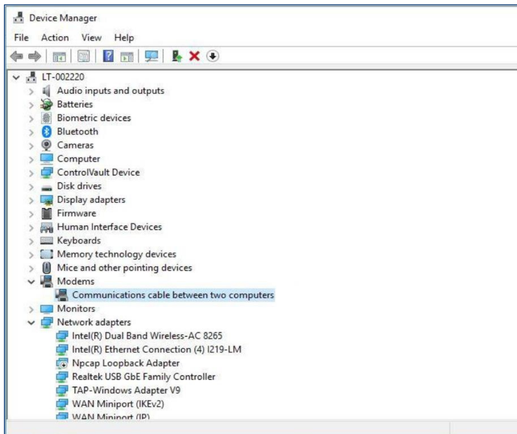
Figure 14. Modem Available
