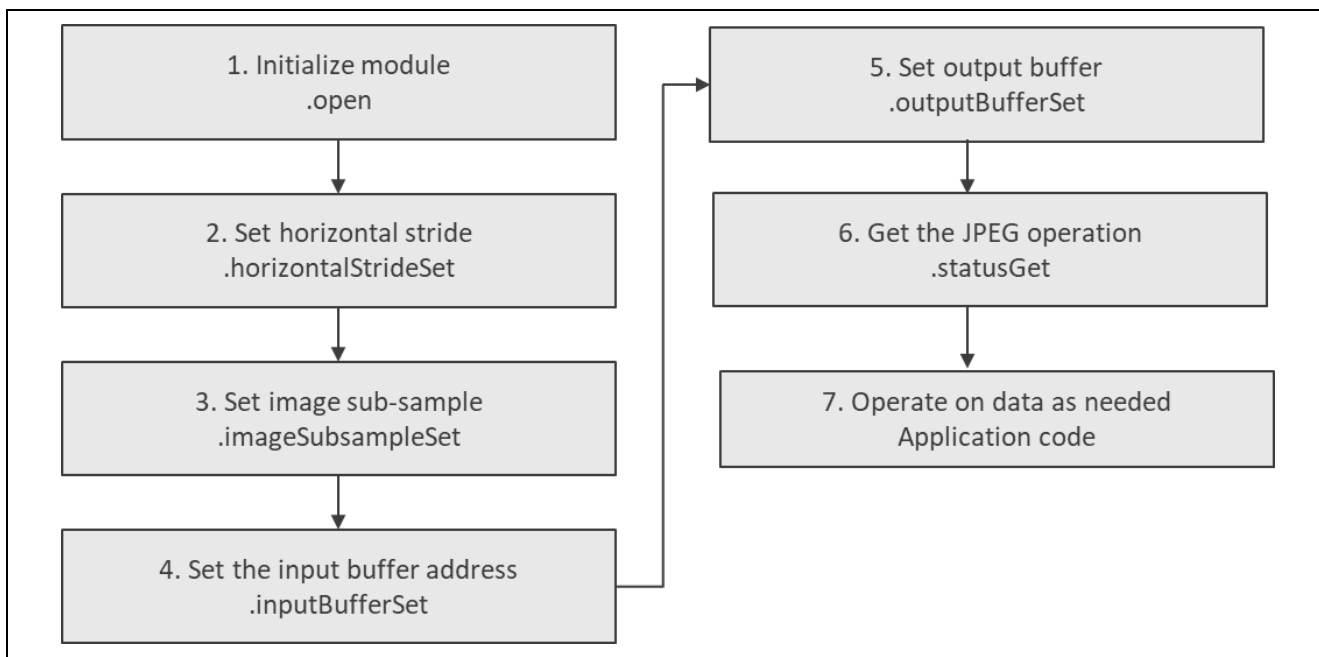
Figure 6. Flow Diagram of Typical Operation
