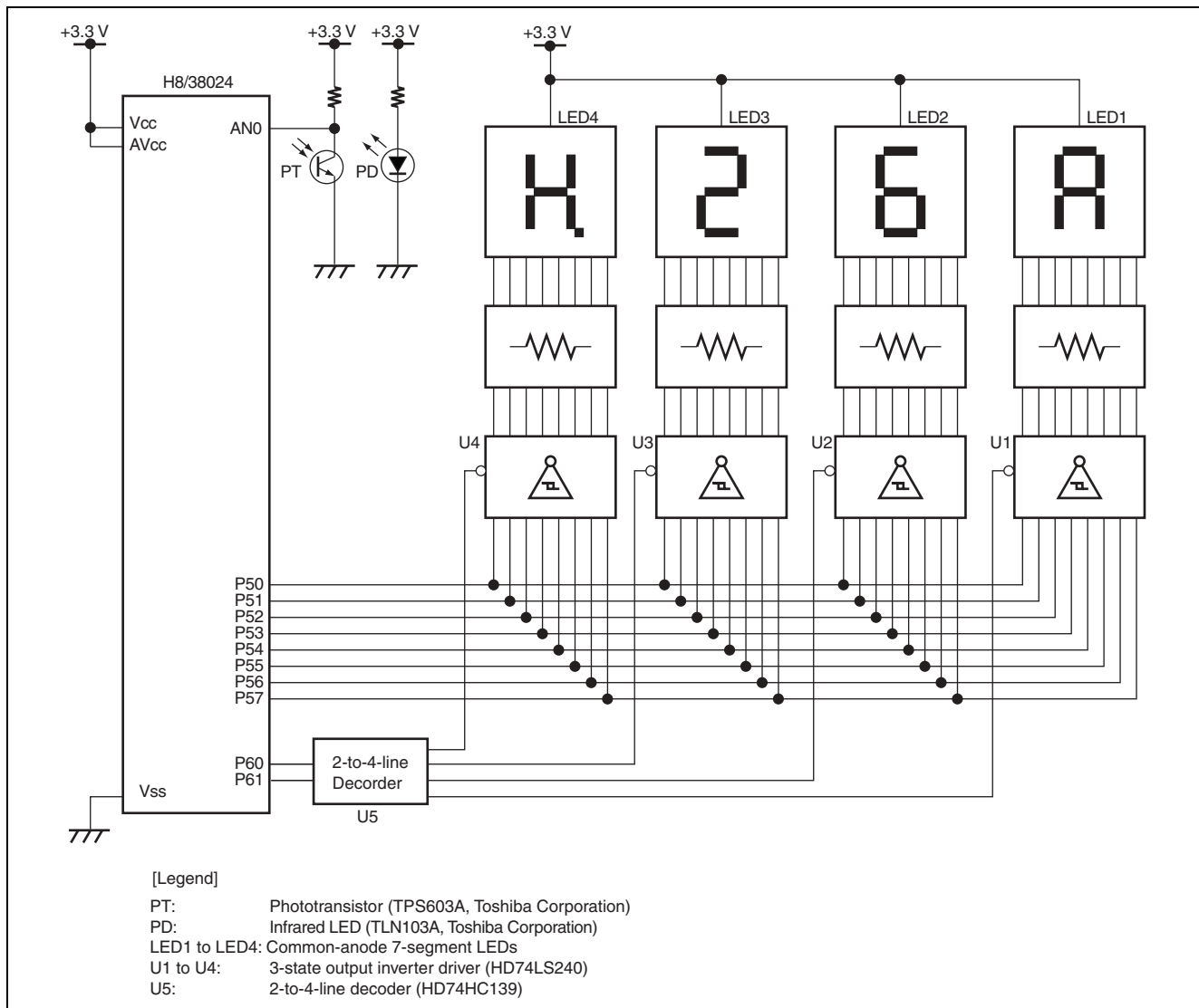
Figure 1.1 Hardware Configuration
