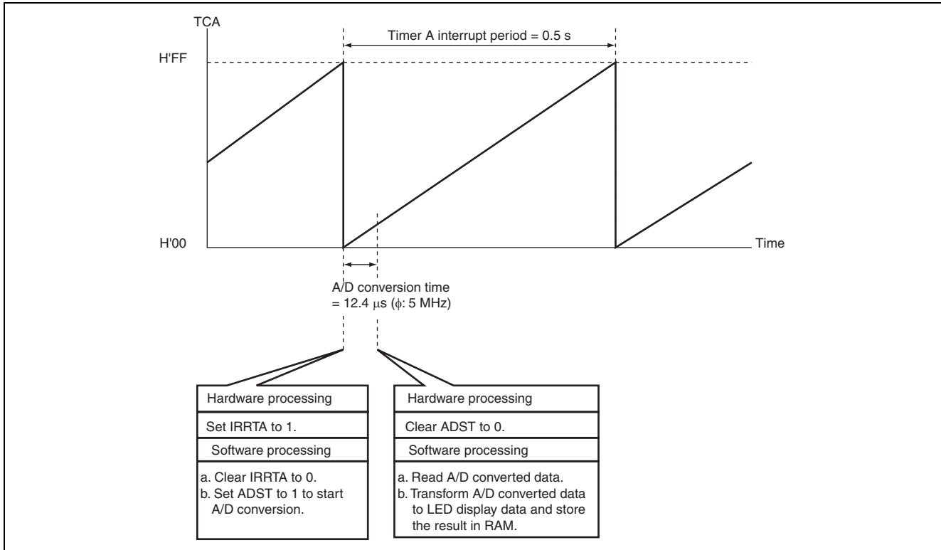
Figure 3.1 Principle of Operation of A/D Conversion of AN0-Pin Signal Using Timer A
