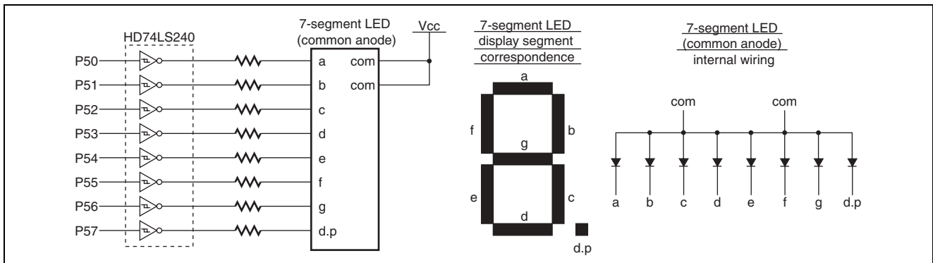
Figure 2.2 7-Segment LED Connections and Internal Wiring
