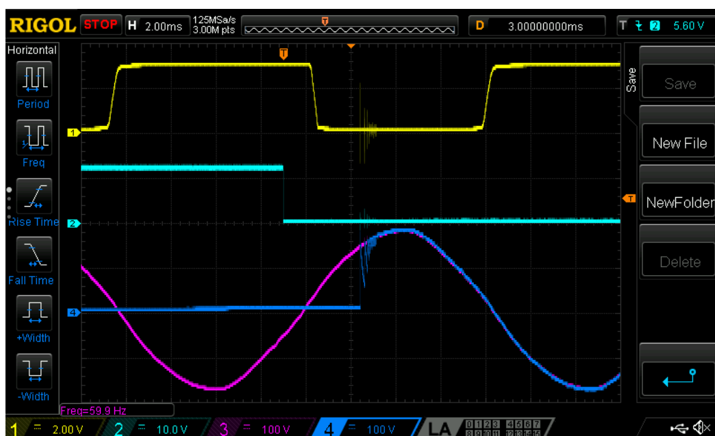
Figure 8: Relay Does Not Close at True Zero-Crossing with 7.407ms Delay
