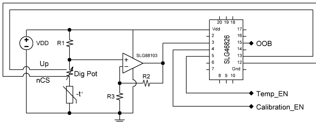
Figure 3: Functional Diagram
