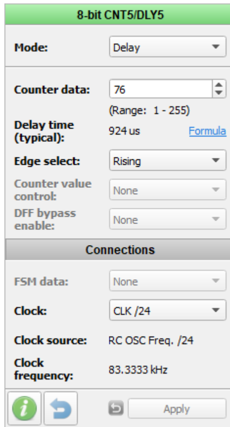
Figure 18: CNT5 Configuration
