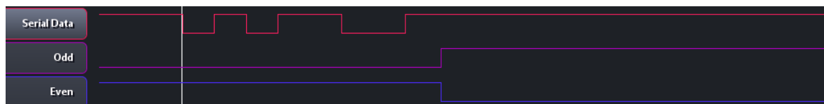
Figure 21: Serial Input Parity Generator Odd Test
