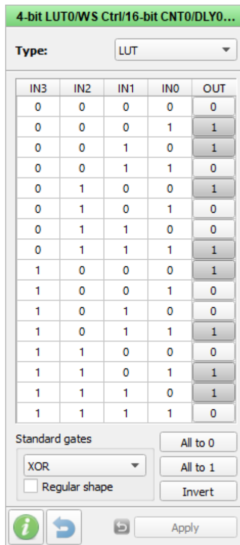
Figure 8: XOR Processor
