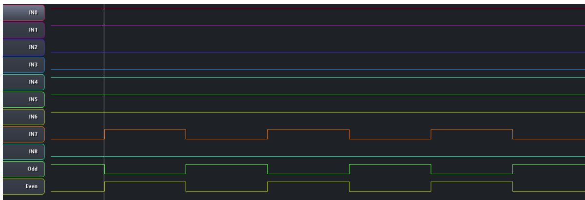
Figure 20: Parallel Input Parity Generator Test
