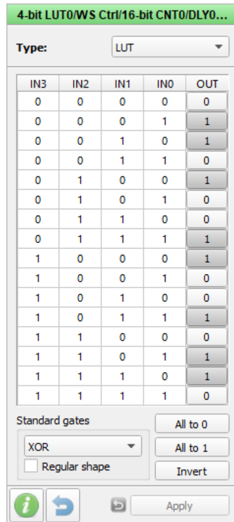
Figure 8: XOR Processor
