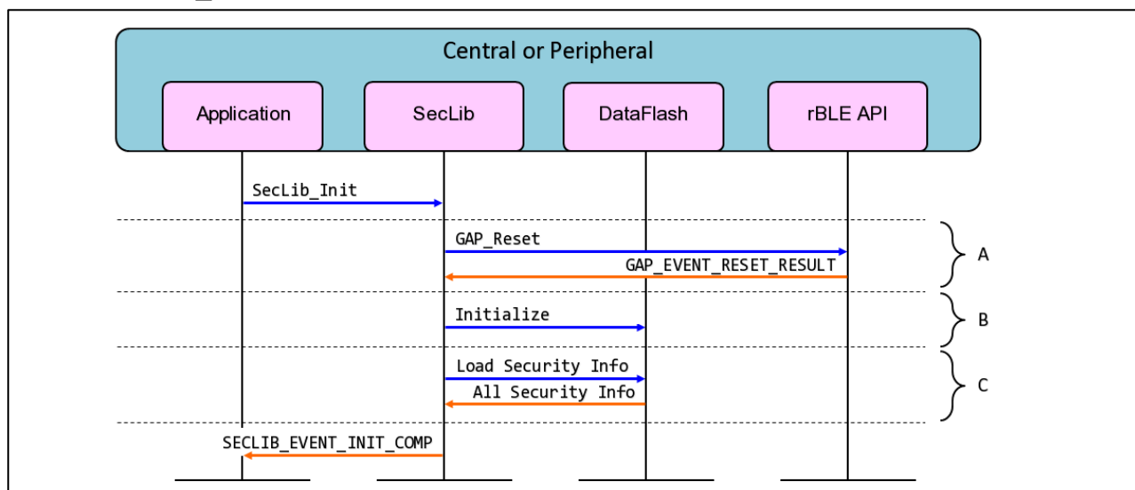
Figure 5-1 Initialization sequence
