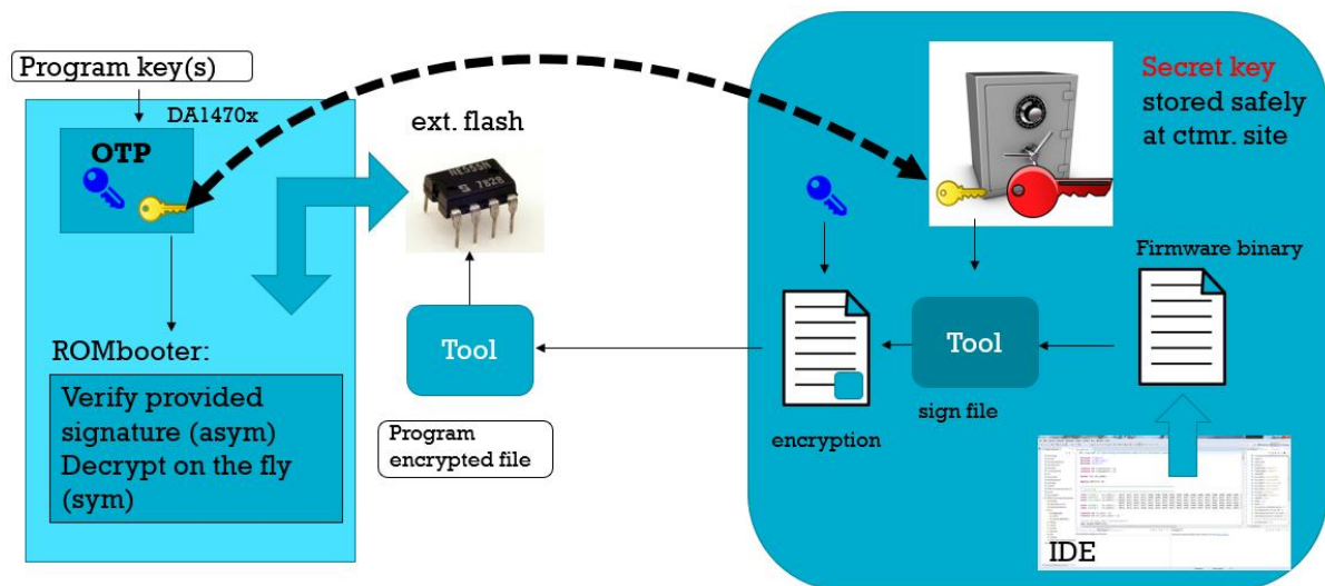
Figure 1: Asymmetric Crypto for Bootloading
