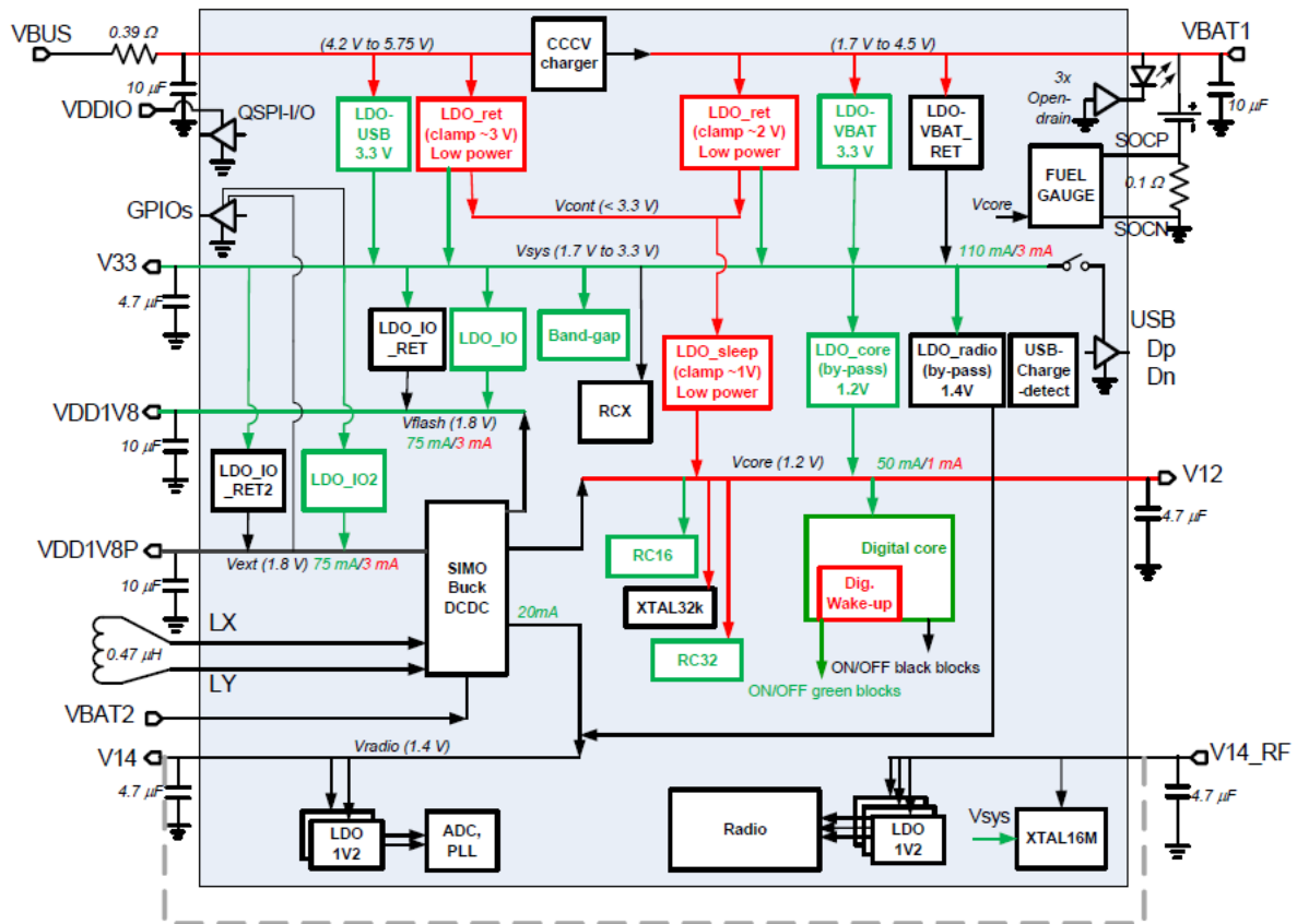
Figure 8: DA1468x power management unit block diagram
