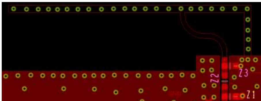
Figure 26: RF matching circuit must be placed as close as possible to the antenna
