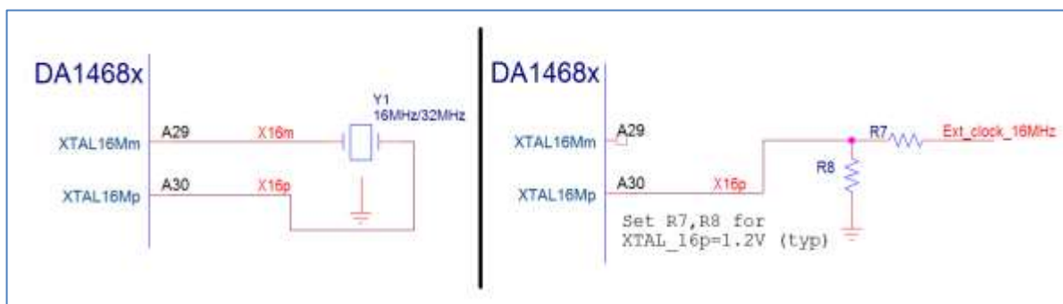
Figure 14: Connection of the crystal (left) and external 16 MHz clock (right) for AQFN package
