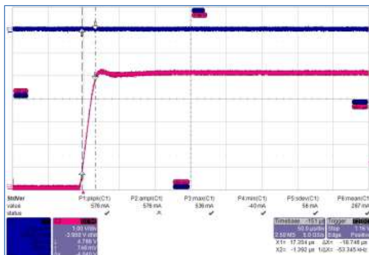
Figure 23: Step response of VBUS with 0.39 \Omega and 10 \mu\text{F} for a 1.5 m USB cable.
