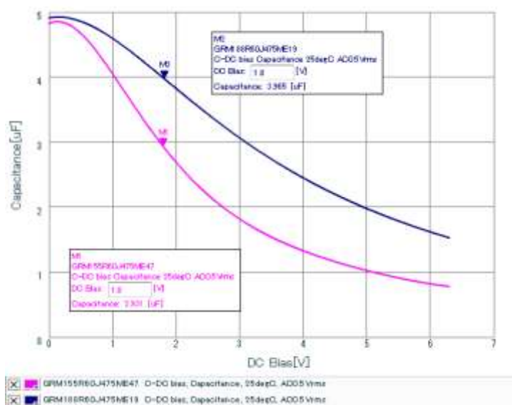
Figure 7: 4.7 \mu F- 6.3V capacitance change for 0402 (purple) and 0603 (blue)
