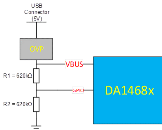
Figure 24: Wakeup from Hibernation by VBUS voltage using GPIO trigger
