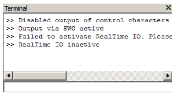
Figure 23 Terminal Window
