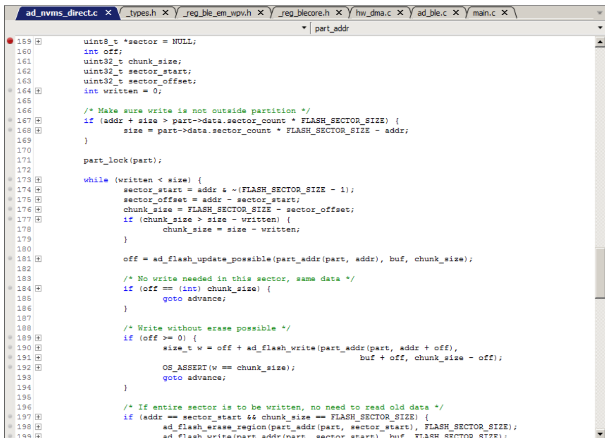
Figure 12 Source Viewer
