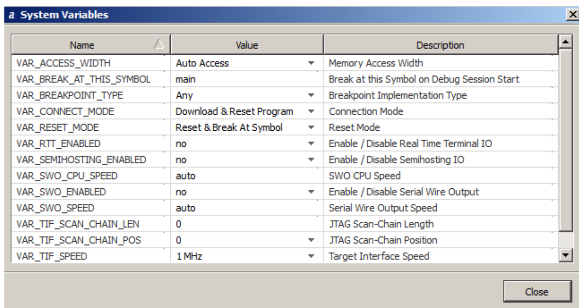
Figure 11 System Variables
