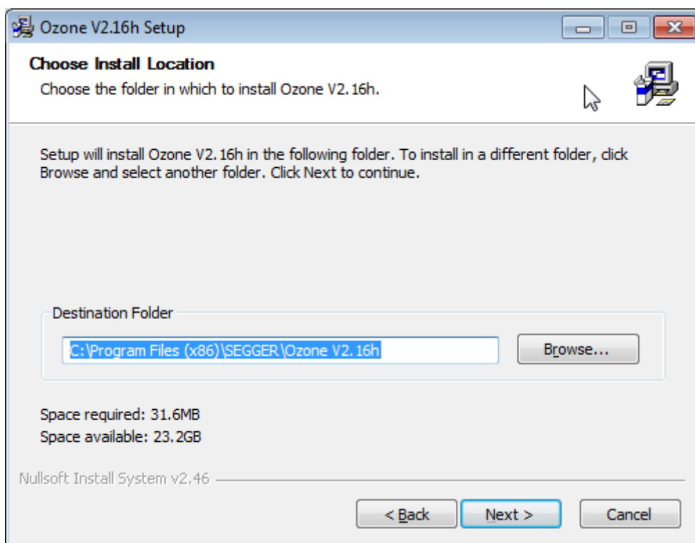
Figure 1: Windows Installer
