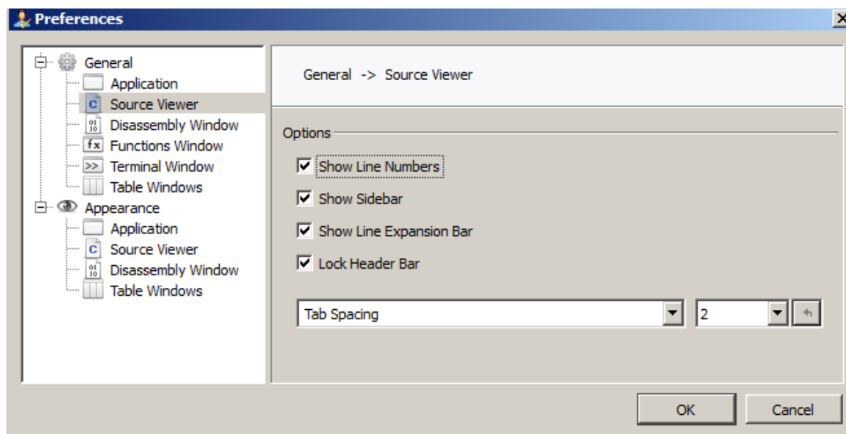
Figure 10 Preferences
