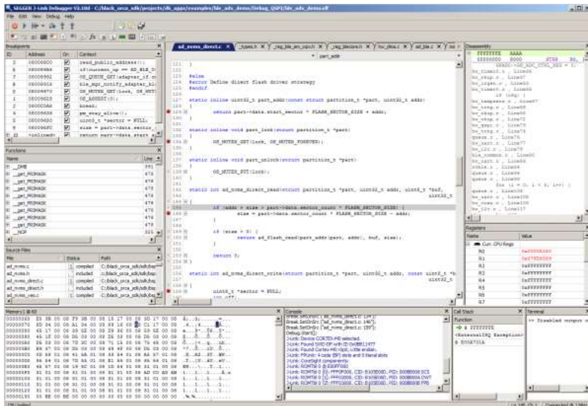
Figure 9 Main Window
