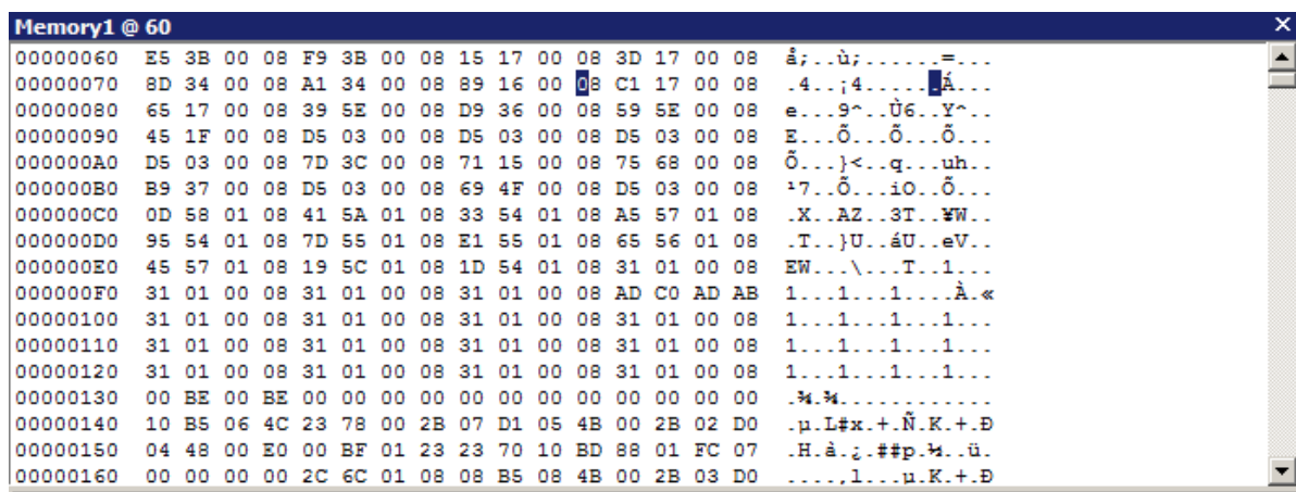
Figure 8 Memory Window
