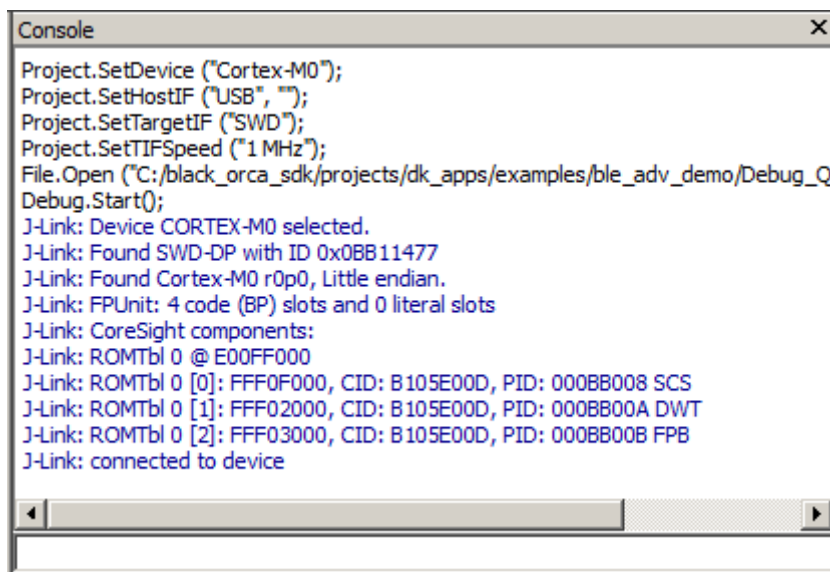
Figure 15 Console Window
