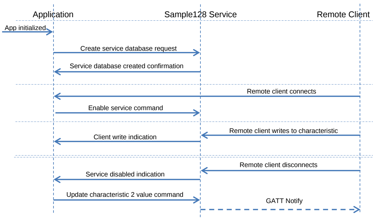
Figure 9: Message flow diagram
