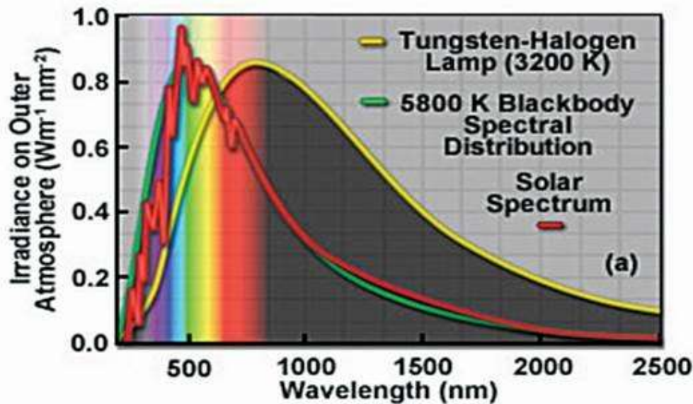
Figure 8: Irradiance plot of a tungsten-halogen lamp and solar light spectrum
