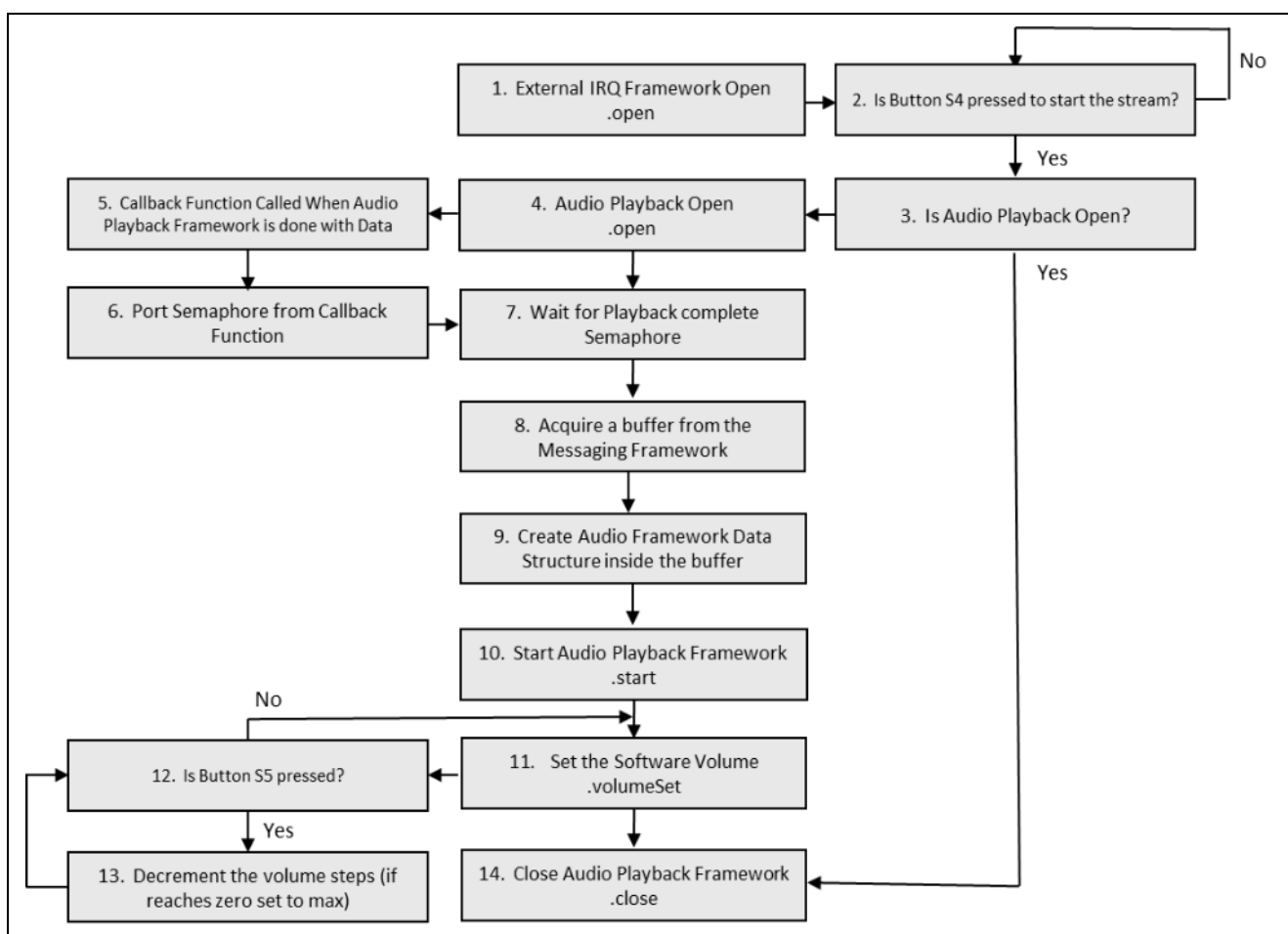
Figure 7. Audio Playback I 2 S Framework Module Application Project Flow
