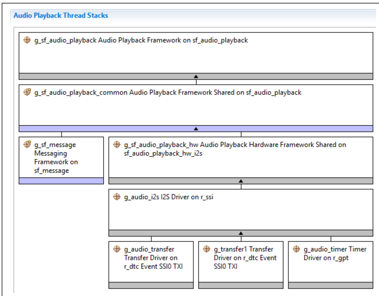
Figure 5. Audio Playback I2S Framework Module Stack
