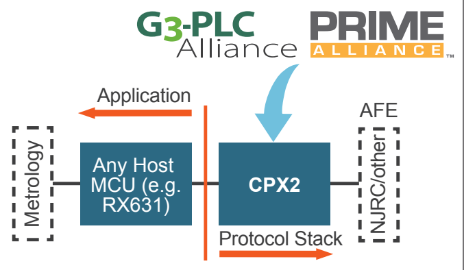
Cool Phoenix 2 System Block Diagram
