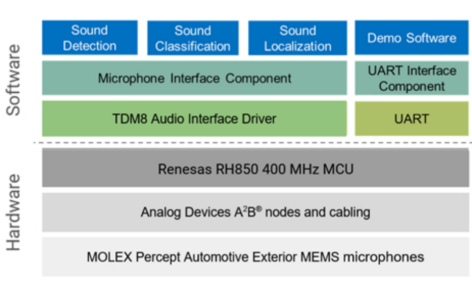
Fig. 5 Reference design HW/SW stack.
