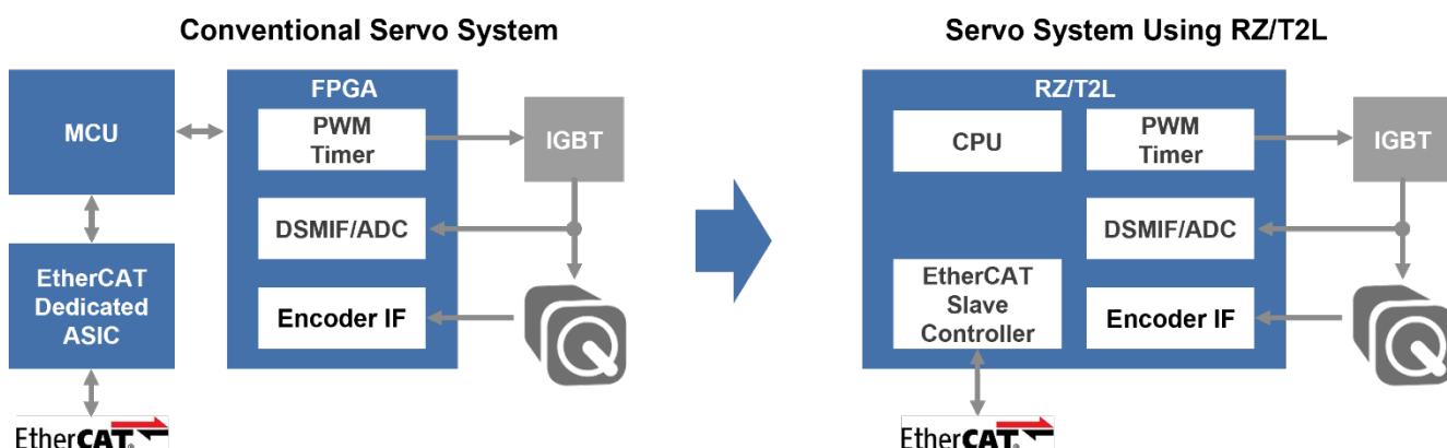
Figure 2: Single-chip AC Servo Solution with RZ/T2L
