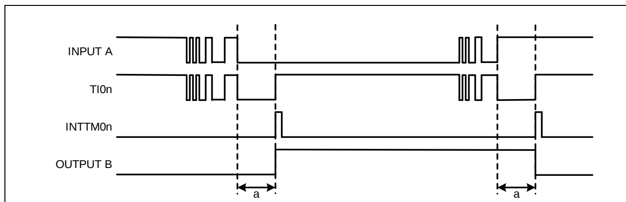
Figure 14. Timing chart
