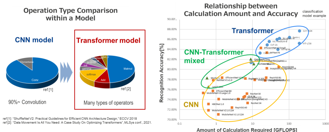
Figure 14: Challenges for Implementing Endpoint AI for Transformer Models
