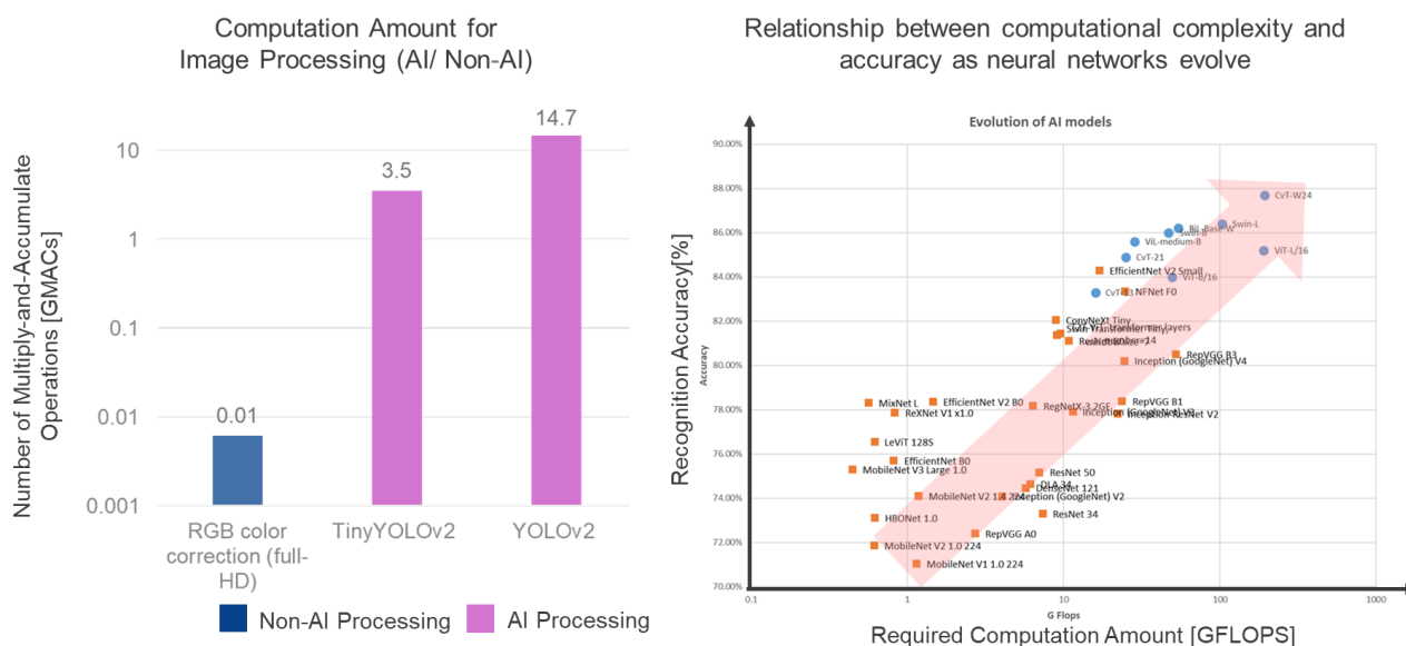
Figure 2: Challenges of Endpoint AI Solutions
