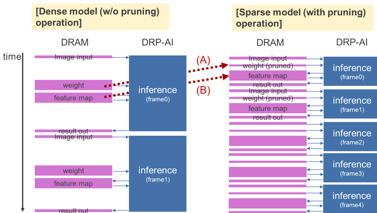
Figure 12: Comparison of Memory Access Between the Pre-Pruning Model (Dense) and the Post-Pruning Model (Sparse)
