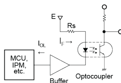
Figure 2. Optocoupler peripheral circuit diagram
