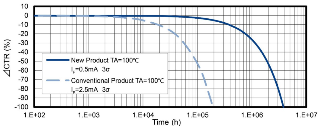
Figure 4. Estimated life
