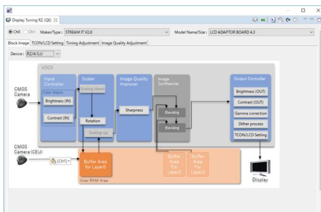
Figure 10 VDC5-based image adjustments with QE Tool
