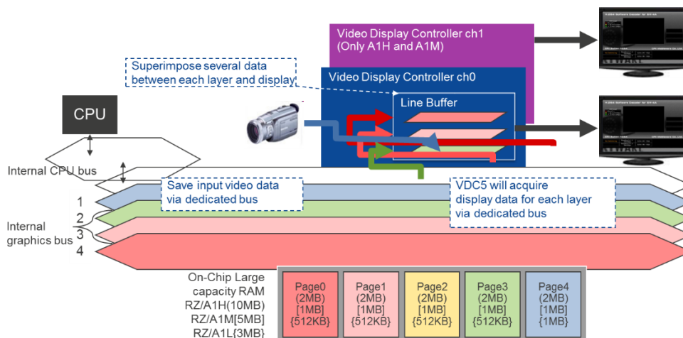
Figure 9 Video and image subsystem of RZ/A1 MPUs
