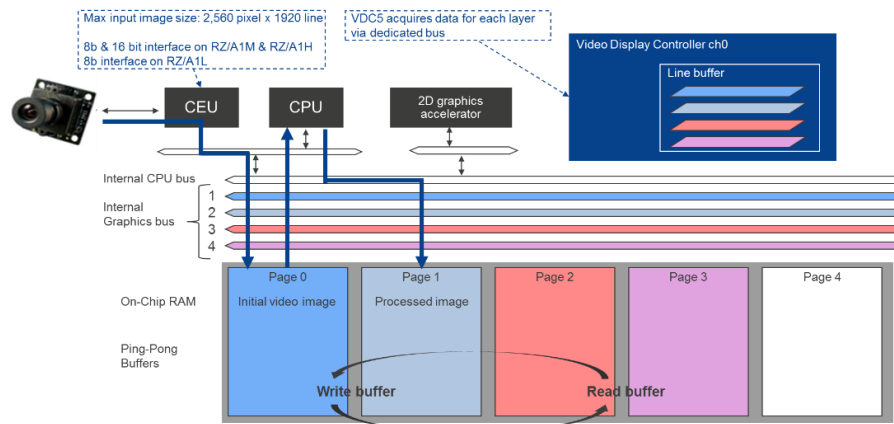
Figure 8 Image capture with CEU and data push to SRAM and VDC
