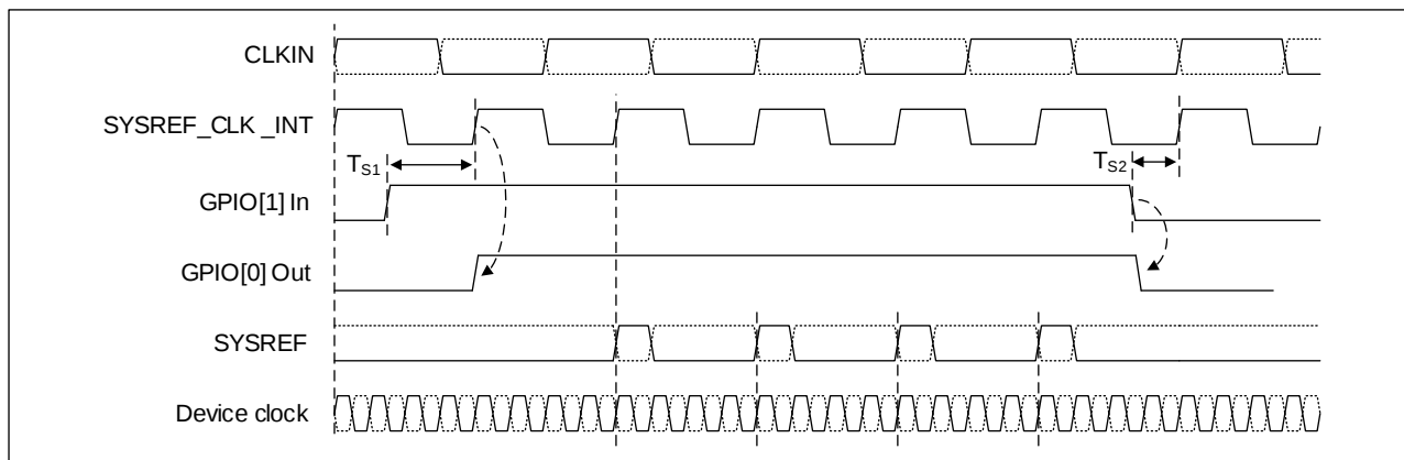
Figure 13. Continuous SYSREF Timing for Primary RC38312
