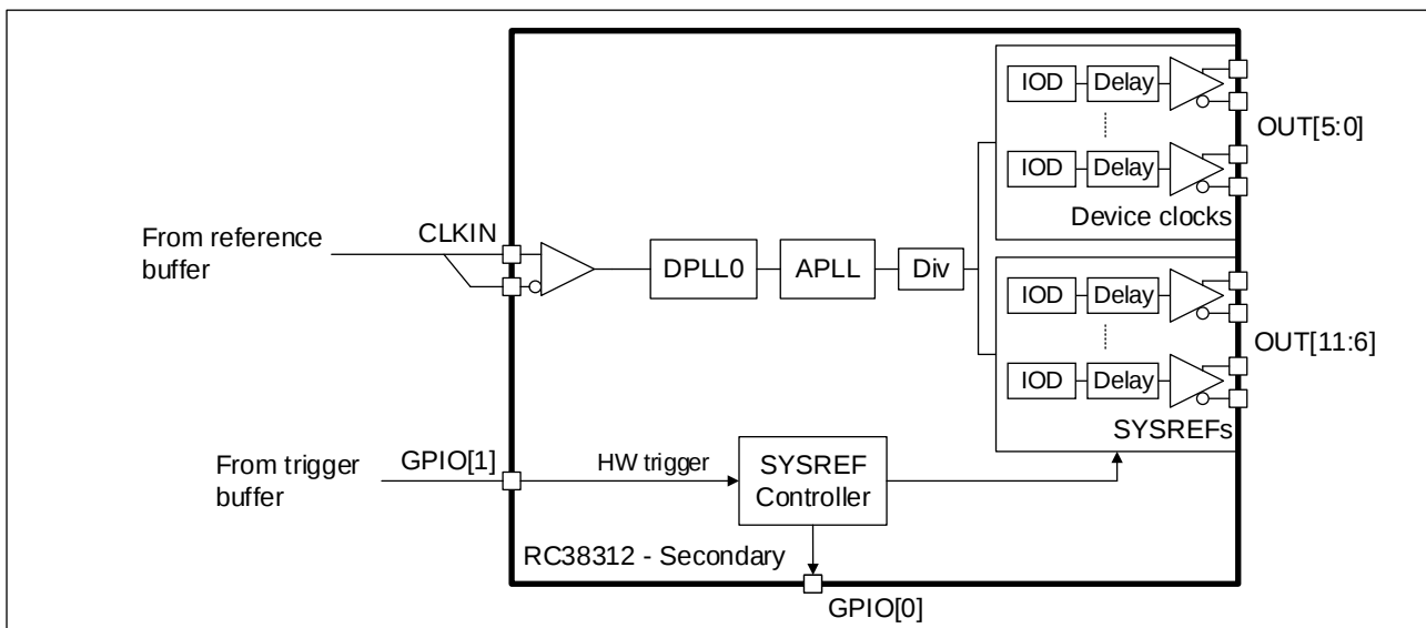
Figure 10. SYSREF Secondary using RC38312
