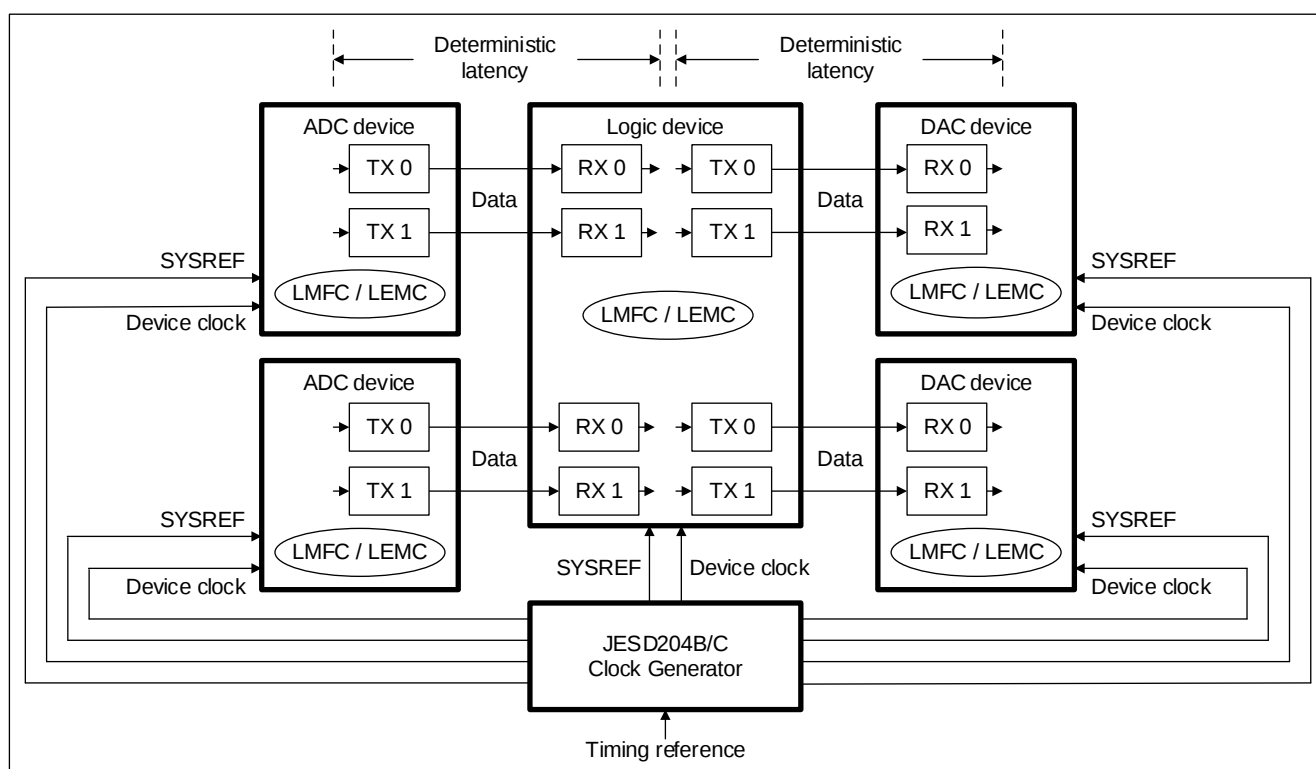
Figure 1. JESD204B/C Deterministic Latency
