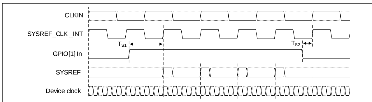
Figure 14. Continuous SYSREF Timing for Secondary RC38312
