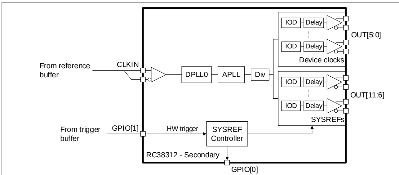
Figure 10. SYSREF Secondary using RC38312
