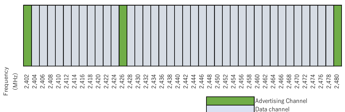
Bluetooth Low Energy Communication Frequency Channels
