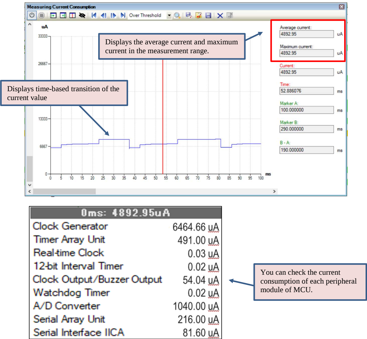
Figure 2-3 Measurement results of current consumption simulation
