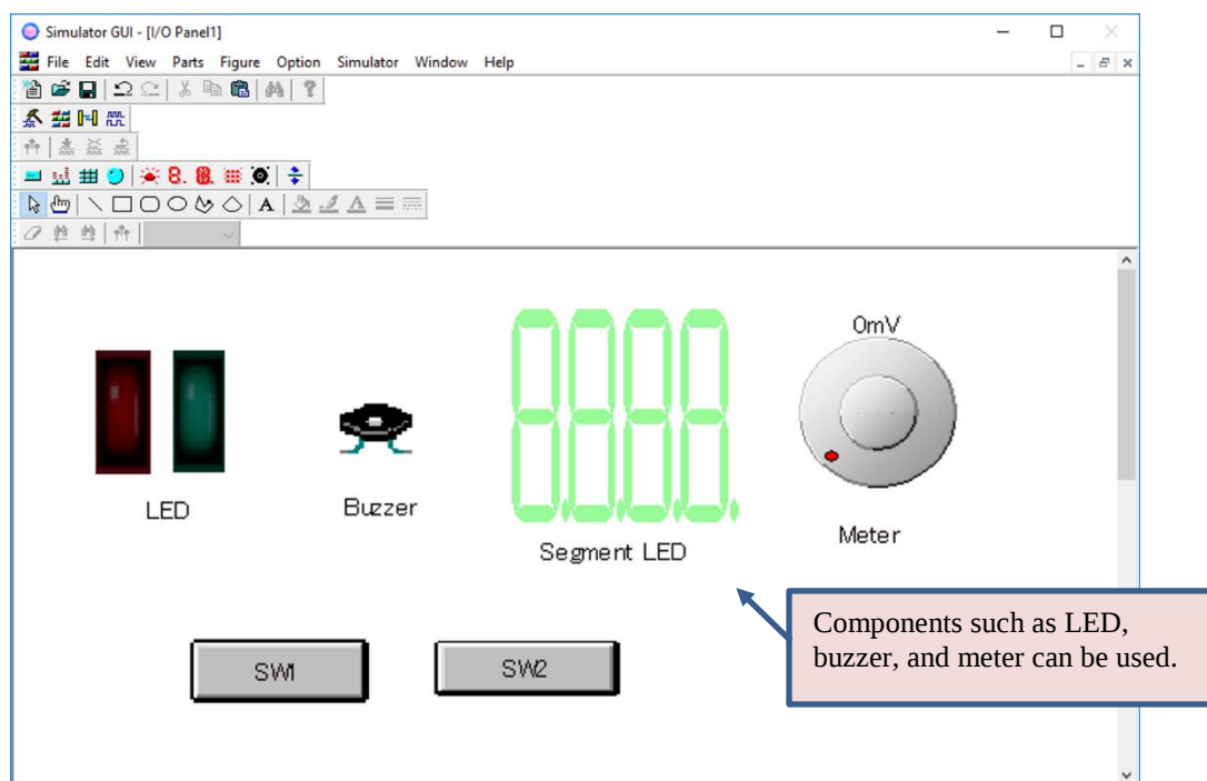
Figure 2-4 Simulator GUI
