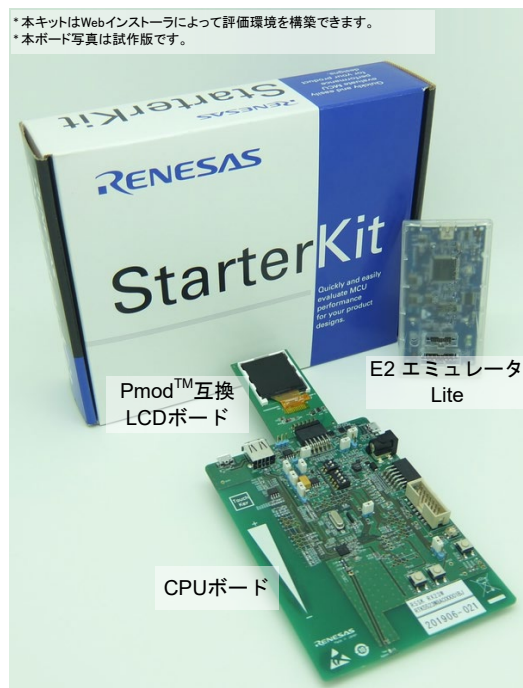
図 1 Renesas Solution Starter Kit for RX23W
