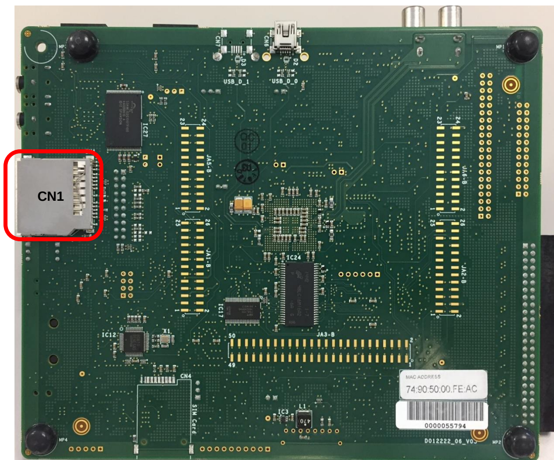
Figure 1 Location of the SD/MMC slot (Solder Side of the Board)
