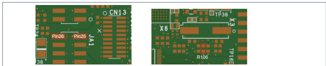
Figure 4 Location of JA1.Pin25 and Pin26 & R106
