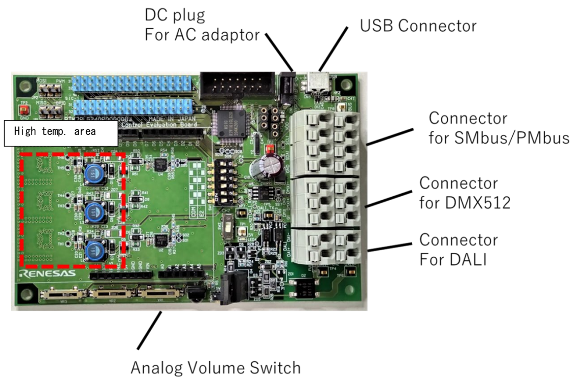
Figure 2-1 Surface appearance (Bottom View)
