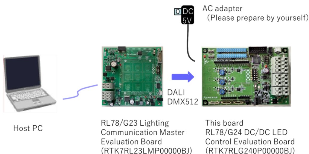
Figure 1-1 Board connection
