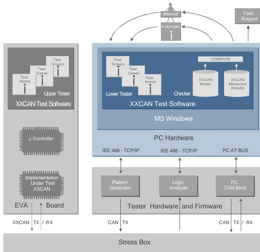
Figure 1: CAN Conformance Test System Overview - © 2000 C&S
