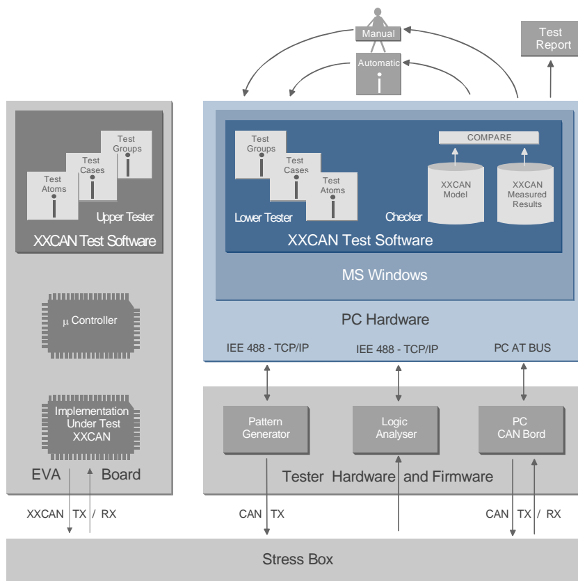
Figure 2-1: CAN Conformance Test System Overview
