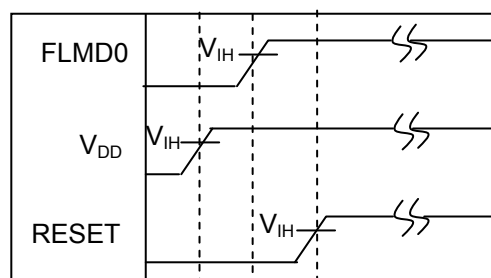
② Entering into flash programming mode at the same time as power-on
