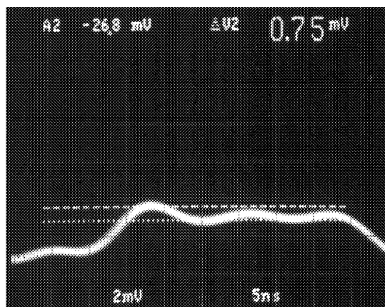
FIGURE 4. GLITCH HEIGHT
