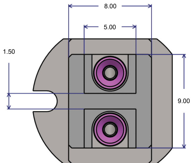
Figure 8. Suggested Power Tower Pickup Tool – Bottom View
