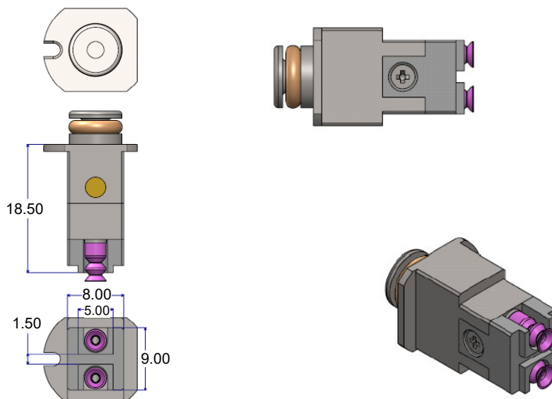
Figure 5. Suggested Power Tower Pickup Tool – Detail 1
