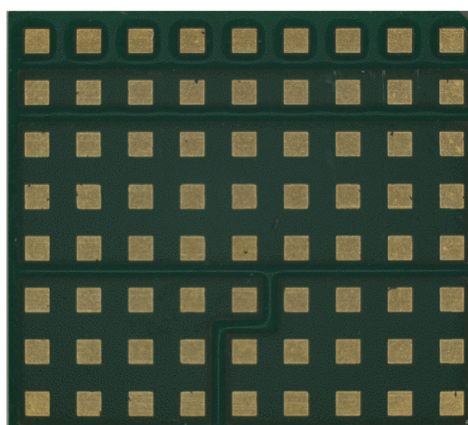
Figure 2. Typical Power Tower Bottom View - RRV29830
