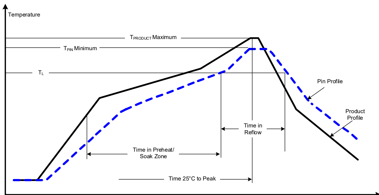
Figure 11. Peak Reflow Profile
