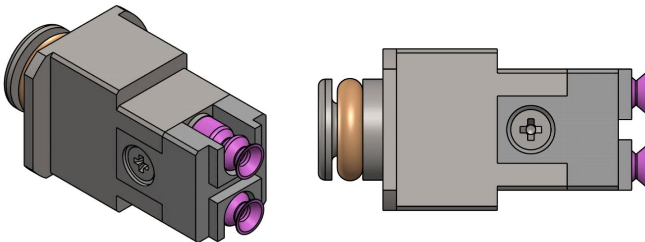
Figure 7. Suggested Power Tower Pickup Tool – 3D and Side View
