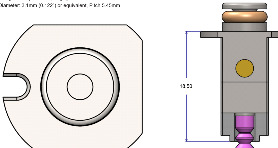
Figure 6. Suggested Power Tower Pickup Tool – Top and Side View
