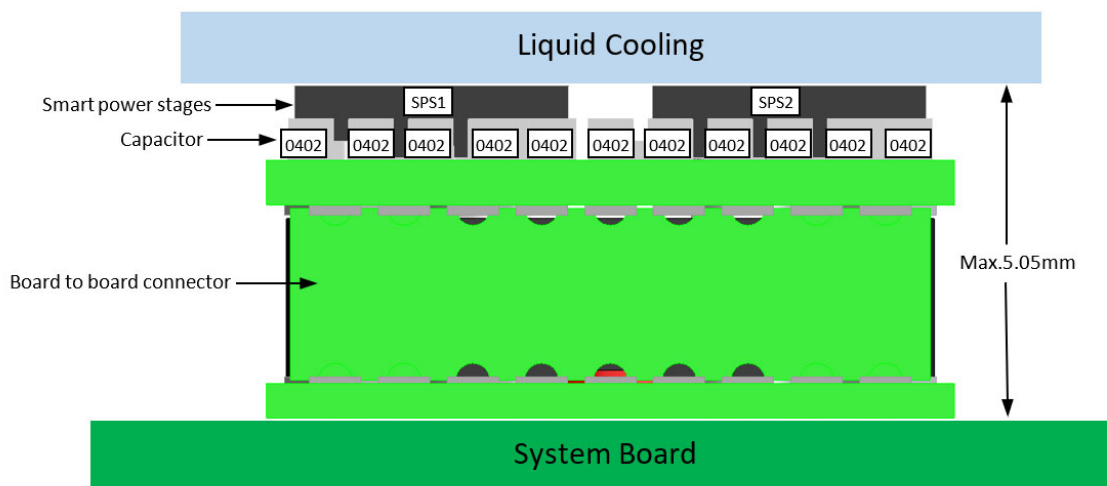
Figure 3. Typical Power Tower Module Cross-Section
