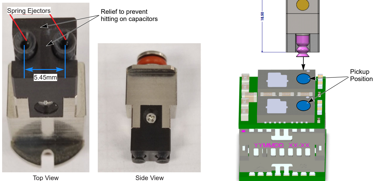
Figure 4. Suggested Power Tower Pickup Tool
