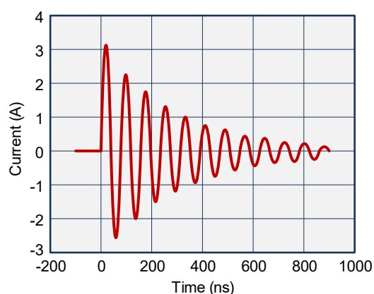
Figure 4. ESD Current During a MM Discharge
