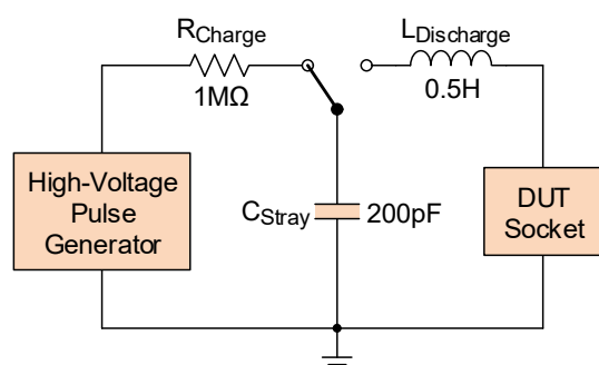
Figure 3. Machine Model
