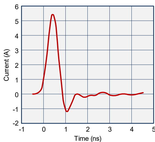
Figure 7. ESD Current During a CDM Discharge
