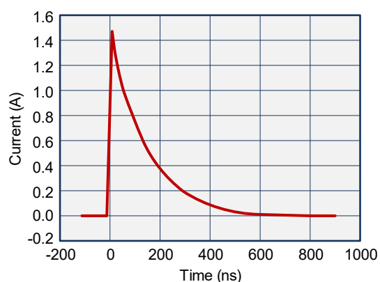
Figure 2. ESD Current During a HBM Discharge
