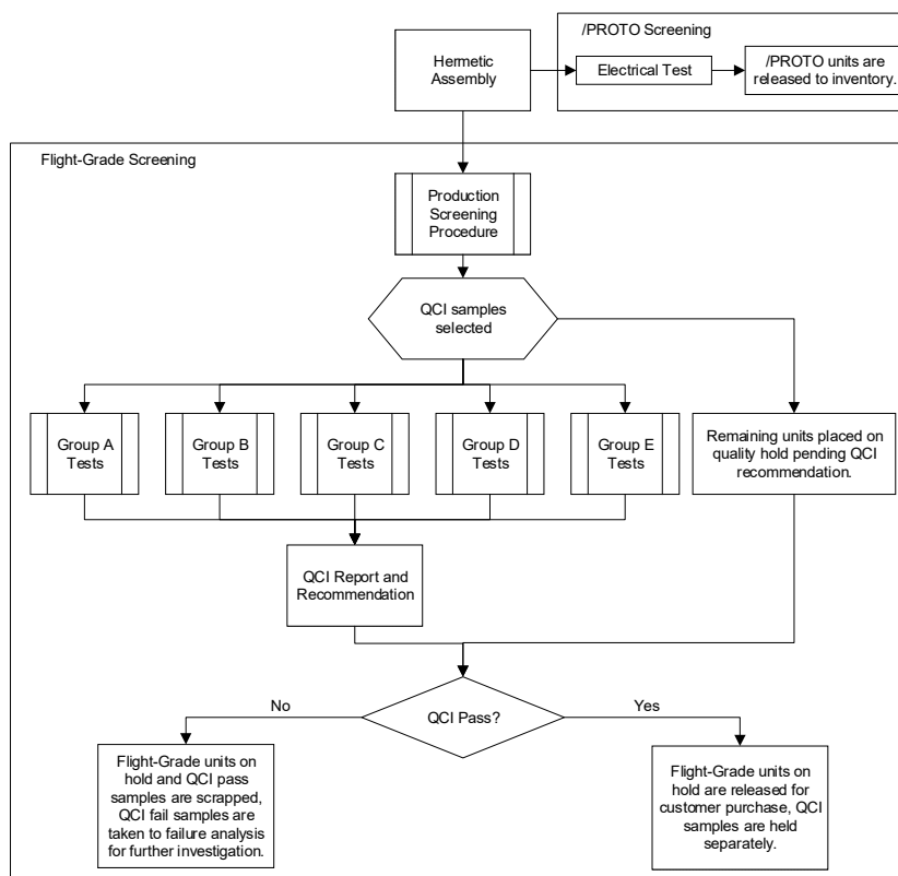
Figure 1. Radiation Hardened QML-V Equivalent Production Flow Chart
