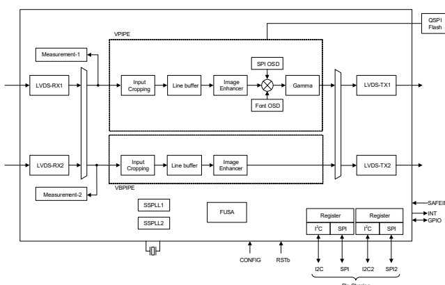
Figure 1. Block Diagram
