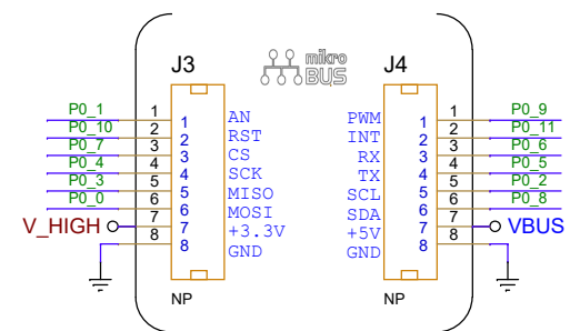
MikroBUS SOCKET (NOT POPULATED)
