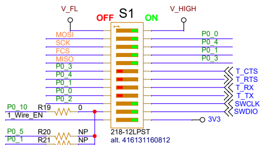
DEVELOPMENT OPTIONS (DEFAULT: FLASH, JTAG, 1-wire UART)
