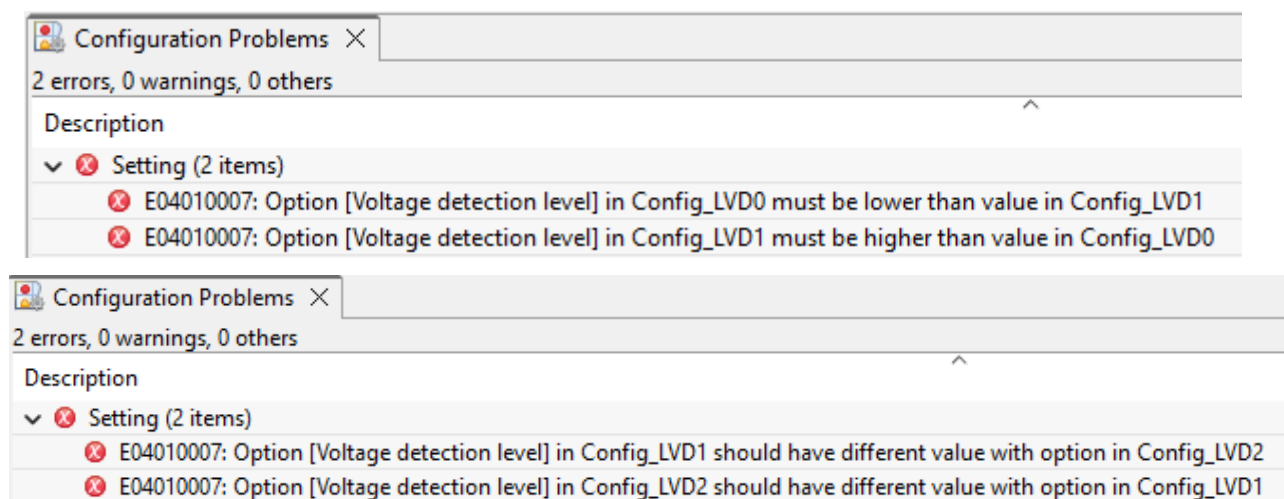
Figure 3-2 The error message is displayed correctly
