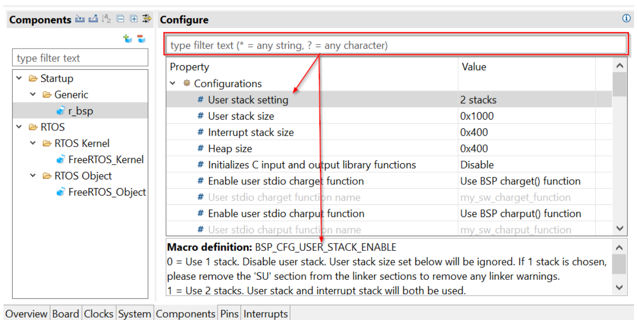
Figure 2-4 Search text box at property grid configuration
