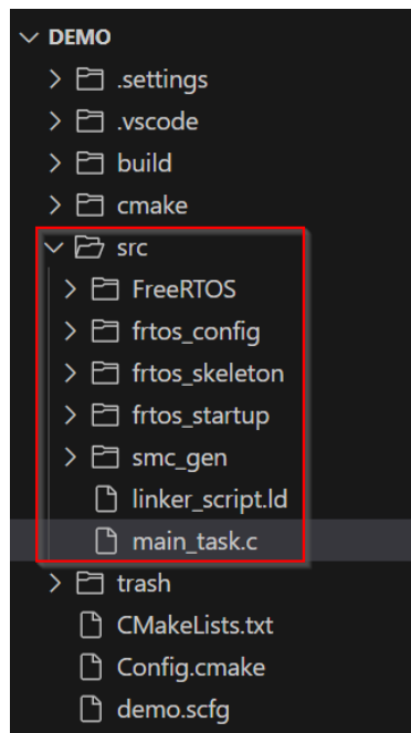
Figure 2-2 Generated project with FreeRTOS kernel selection
