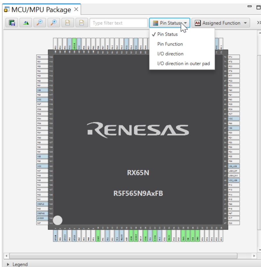
Figure 2-2 MCU/MPU Package view with outer pad setting
