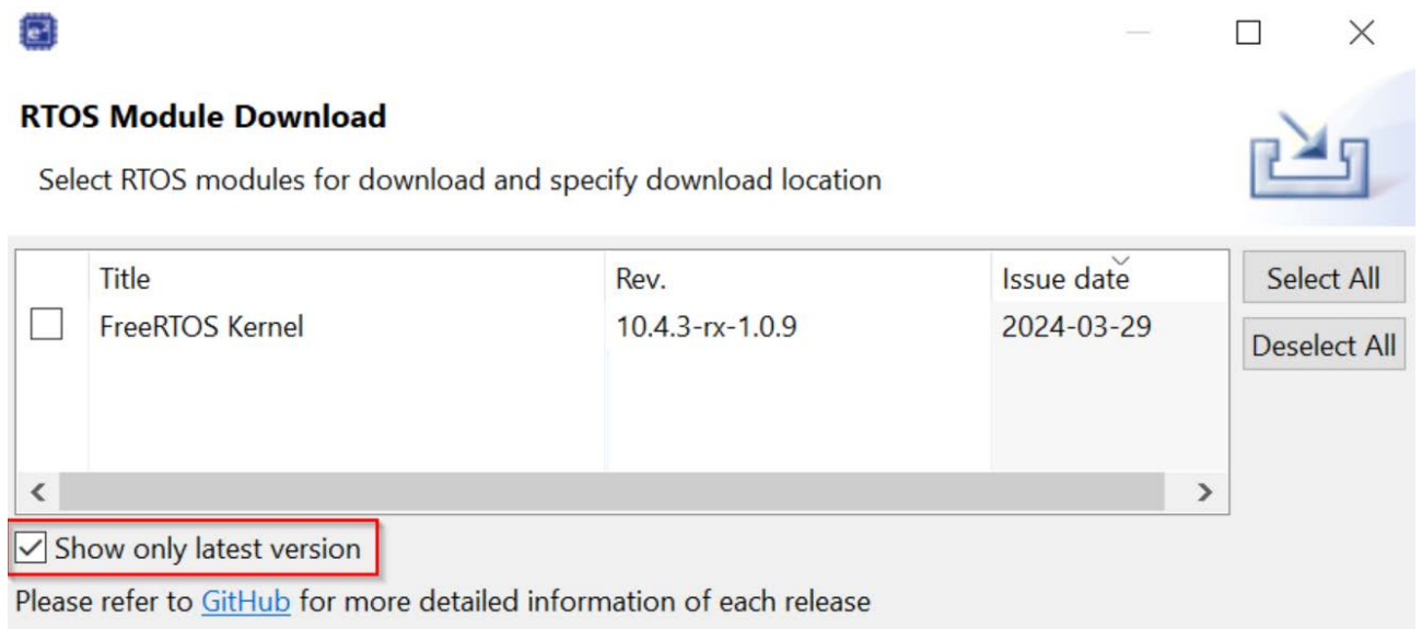
Figure 2-4 FreeRTOS Kernel download dialog
