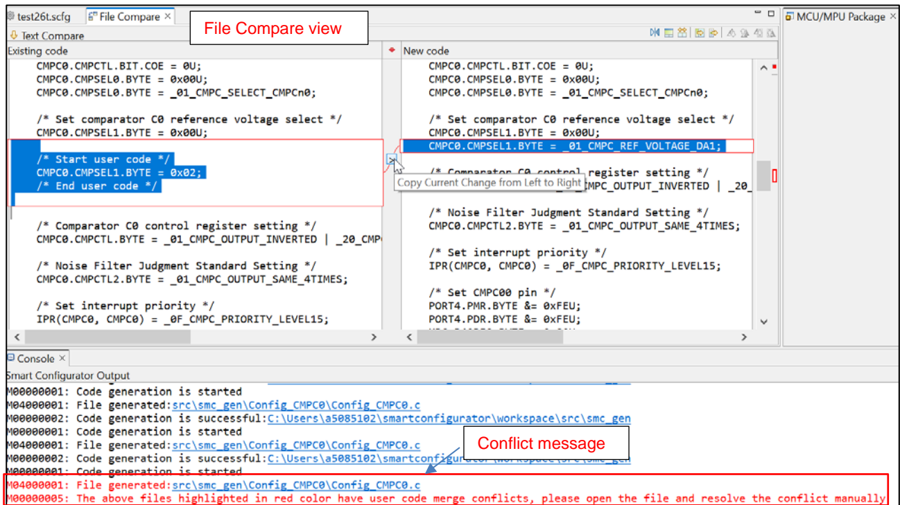
Figure 2-4 Compare view for generated files with user codes merge conflicts.
