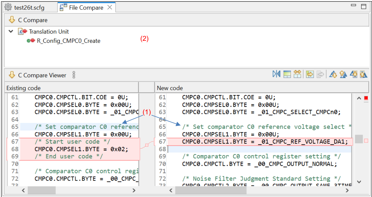
Figure 2-5 Compare view for generated files with user codes merge conflicts in e2 studio.
