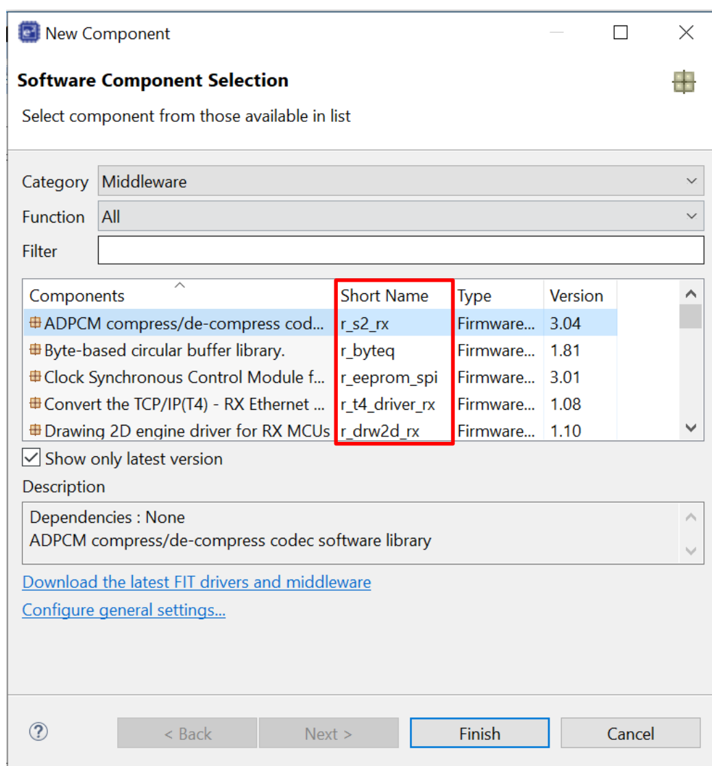
Figure 2-3: New “Short Name” column for FIT component
